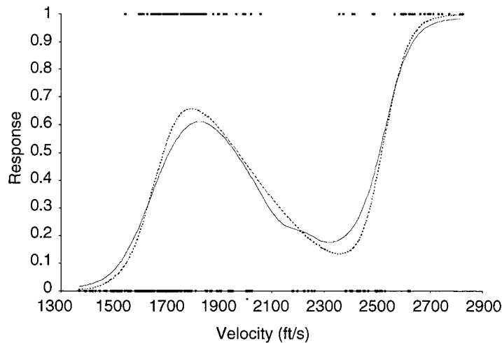
Figure 3. Comparison of fits between llogrs (solid line) and cdf mixture model (dashed line).
