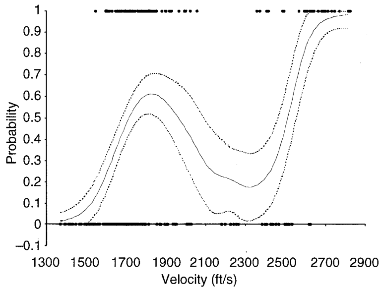
Figure 4. Local logistic regression fit to macrocomposite data with 95% confidence bands.
