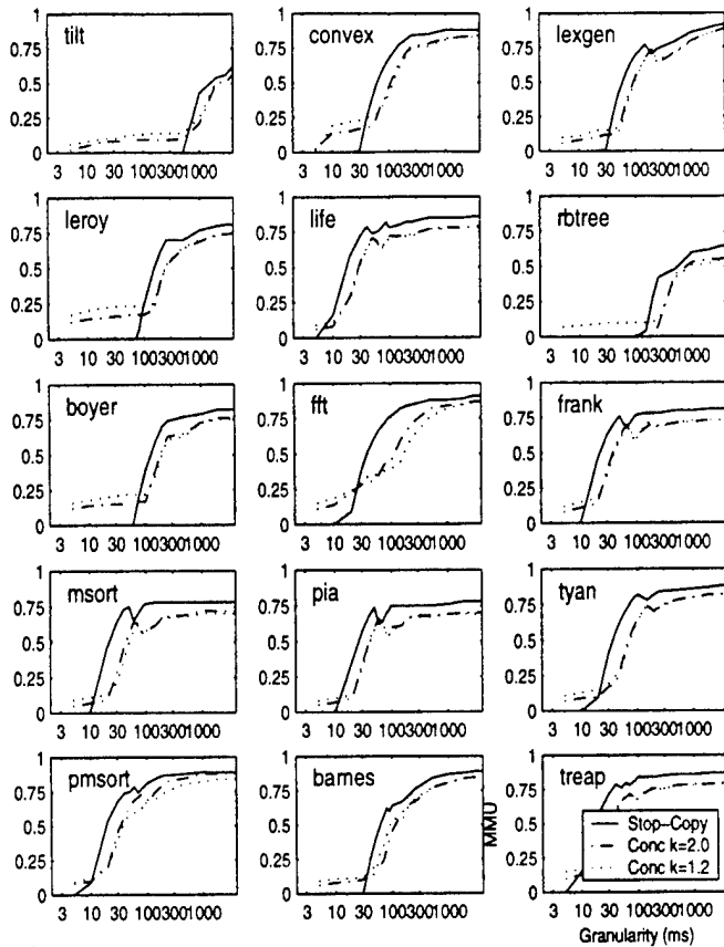
Figure 2: MMU vs granularity (ms) of semispace collectors: non-incremental, incremental ( k=1.2 ), and incremental ( k=2.0 )
