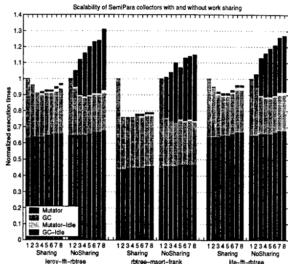
Figure 5: Total processor time spent in various states for finely parallel benchmarks.
