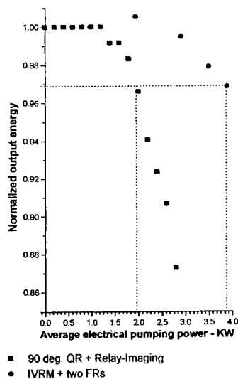
Figure 5: Normalized output energy from birefringence compensated polarized resonators using either an inter-rod 90^\circ QR + relay imaging or two FRs + IVRM + relay-imaging.
