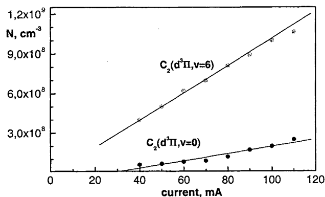
Fig.6. Concentration of \text{C}_2(d^3\Pi, v=0) and \text{C}_2(d^3\Pi, v=6) vs discharge current He+12%CO, p=15 Torr
