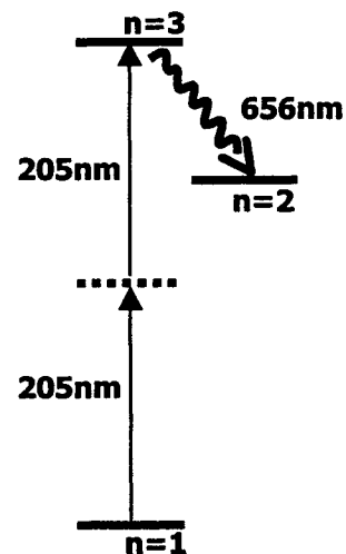
Figure 1 Energy level diagram showing the pump and fluorescence transitions used in the TALIF scheme.
