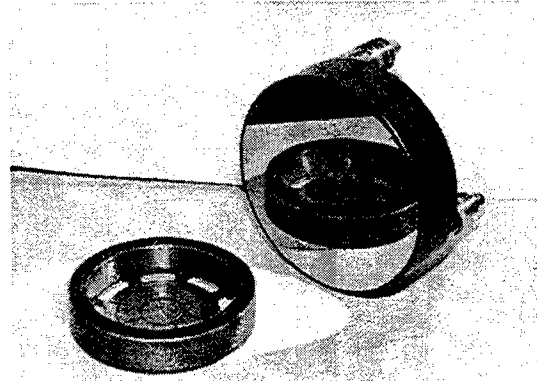
Fig. 3. A photo of a sample of a water cooled bimorph corrector
