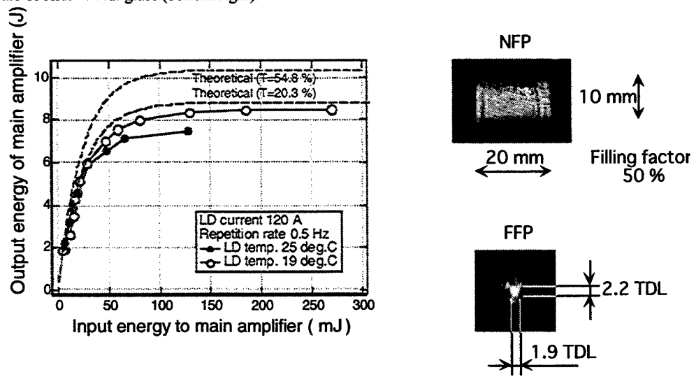
FIG. 9. 1053-nm output energy at 0.5 Hz versus input energy (left), and near field(NFP) and far-field (FFP) patterns at 8.5-J output energy at 0.5 Hz (right).
