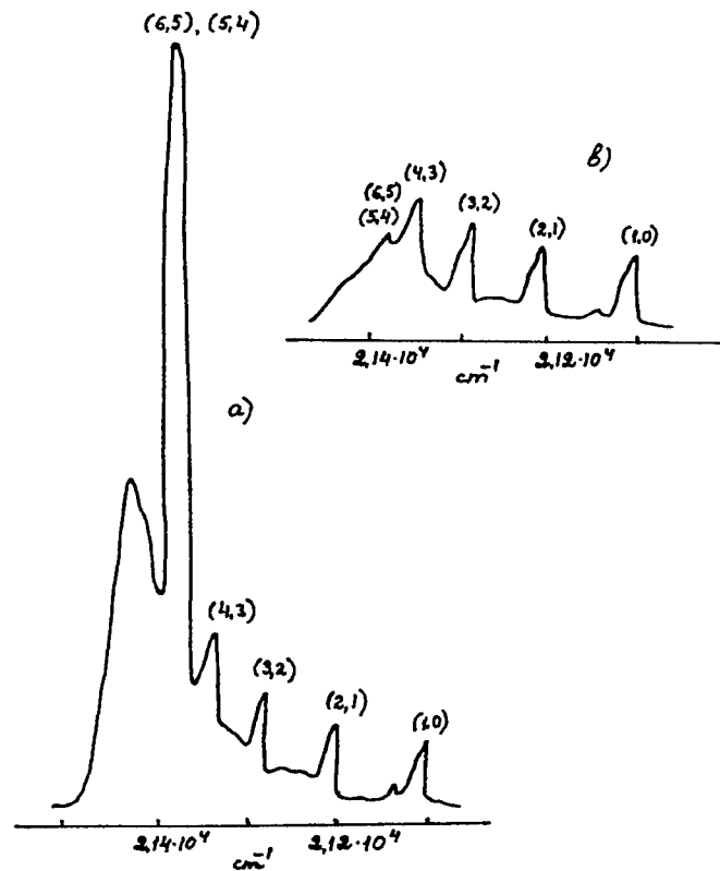
Fig.5. The spectrum of Swan bands of C 2 (d 3 Π → a 3 Π, Δv = 1):
