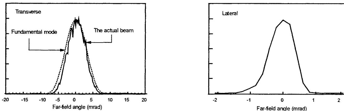
Fig. 4 Far-field profiles of the output beam (10 \mu s pulse width, 1 kHz pulse rate) from the 7-pass waveguide amplifier
