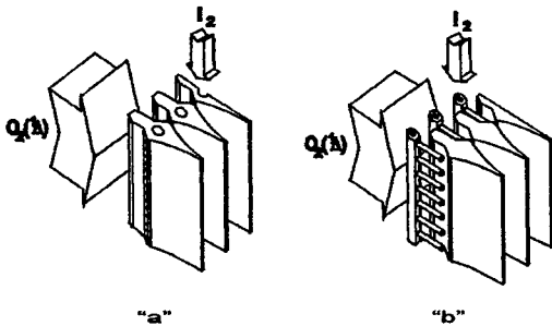
Fig. 2. Supersonic COIL’s mixing systems: “a” – traditional mixing system with transverse iodine injection into singlet oxygen flow through holes in the nozzle’s walls, “b” – mixing system with iodine injection in parallel to singlet oxygen flow through thin tube injector.
