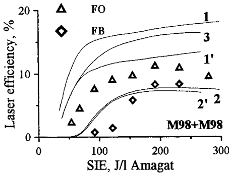
Fig.6. Laser efficiency vs. specific input energy (SIE) for mirror set M98+M98 (experiment -points; theory -curves) Theoretical results: 1, 1', 3 - first-overtone (FO) lasing; 2, 2' - fundamental band (FB) lasing 1, 2 - base model; 1', 2' - additional nonselective optical losses are included (0.5% per single pass); 3 - FB lasing is assumed to be suppressed, additional optical losses are the same CO:N 2 :He=1:9:10; N=0.12 Amagat; SIE=300 J/l Amagat; T=100 K 9
