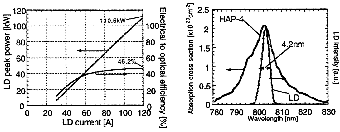
FIG.8. Photograph of quasi-CW 110 kW AlGaAs laser diode module (top), measured total peak power and electrical to optical efficiency (bottom left), and comparison between measured lasing wavelength of module and absorption line of HAP-4 Nd: glass (bottom right).
