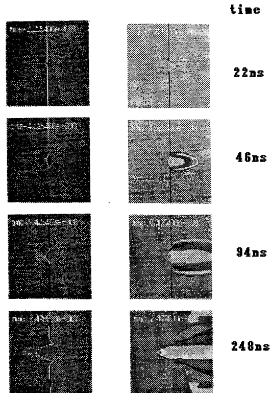
Fig.4 Density (left) and temperature (right) contours of ablated graphite with short pulse KrF laser light.
