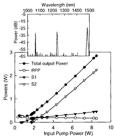
Figure 4 Power evolution of Total power, Residual pump power (RPP) and first Stokes ( S_1 ) and second Stokes ( S_2 ) power in the FSRFL. Inset shows the total output spectrum
