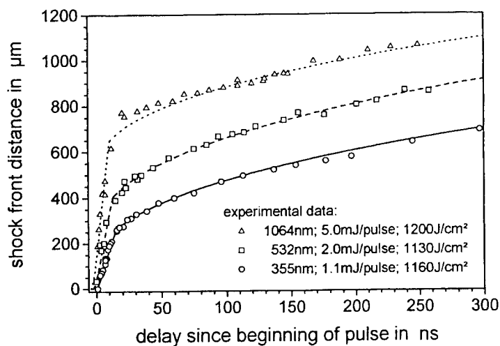
Figure 4. Axial shock front expansion for three different processing wavelengths of a Nd:YAG-laser. Target material Si 3 N 4 ; ambient gas: air, 0.1 MPa. The experimental data has been analyzed by modified models of 2-dimensional LSD-wave propagation ( \lesssim 15 ns) and of gasdynamic blast wave expansion ( \gtrsim 15 ns).
