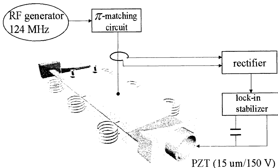
Fig. 1. Experimental setup for the stabilization of RF excited slab \text{CO}_2 laser.
