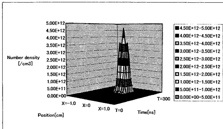
Fig.6 Photon number density
