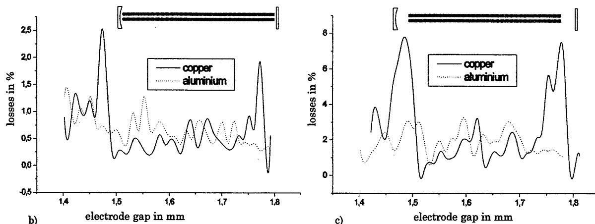
Fig. 5a and 5b: Losses versus electrode gap for the lowest-loss mode applying different mirror-guide distances
