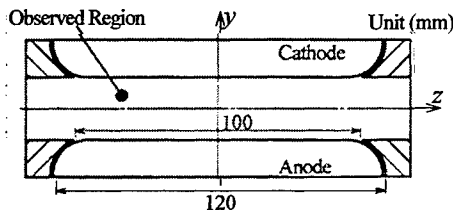
(c) Cross-sectional view of electrode (y-z plane).
