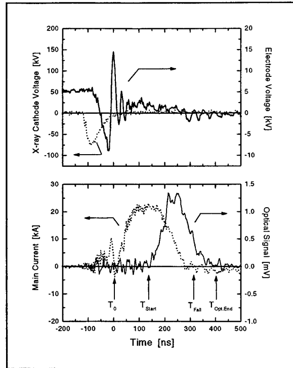
Fig.4 Typical waveforms of the laser pulse
