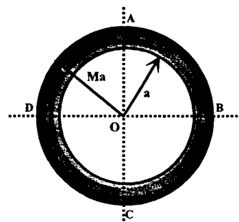
Fig. 5 Beam cross-section of UR90 with annular beam on the scraper mirror position
