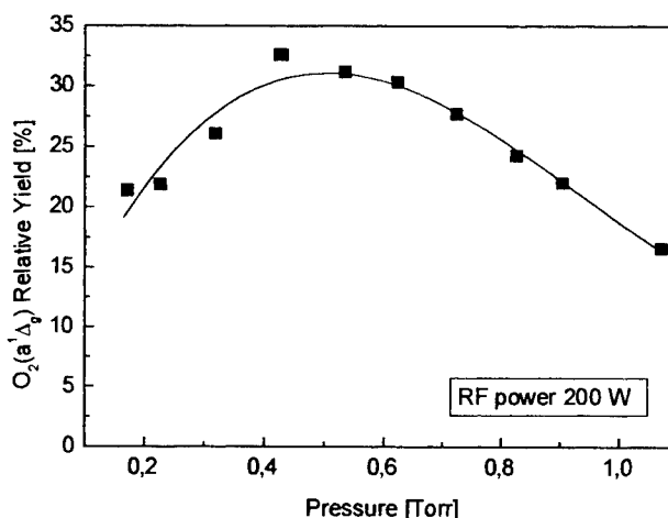
Fig. 3 O 2 (a 1 Δ g ) relative yield vs. pressure
