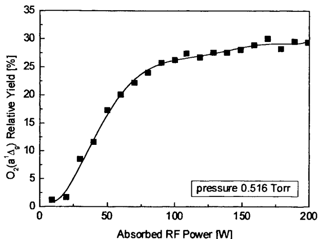
Fig. 2 O 2 (a 1 Δ g ) relative yield vs. RF power
