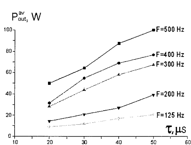
Fig.4. Dependencies of average output power of laser generation vs. pumping pulse duration and pulse repetition rate.
