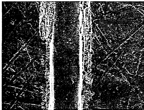
Fig. 2: Typical recast layers in percussion drilling of 1 mm thick steel with ns lasers. The total recast with thickness up to several tens of micrometers is composed of about 1 \mu m thick layers
