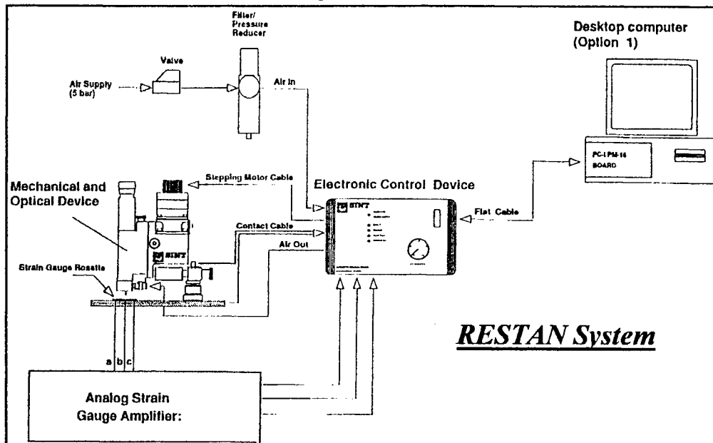
Fig.1 Instrumentation layout
