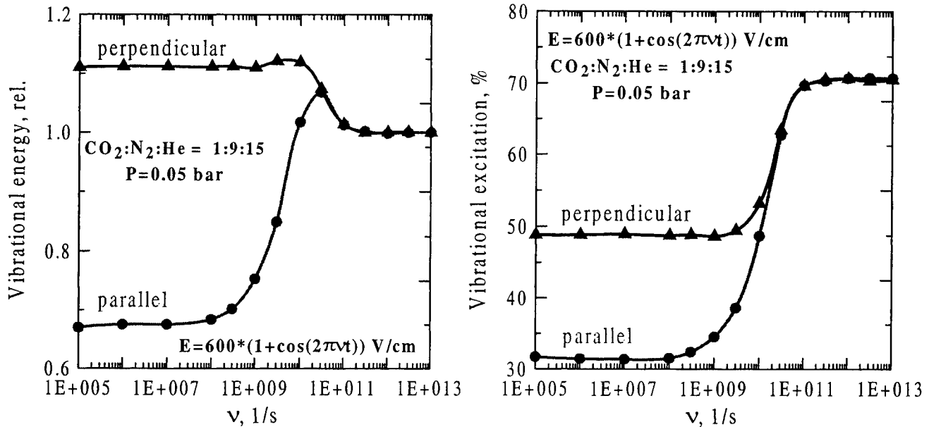
Fig. 3. (a) Energy transferred to the vibrational modes of nitrogen and (b) its ratio to whole absorbed energy in DC +HF plasma.
