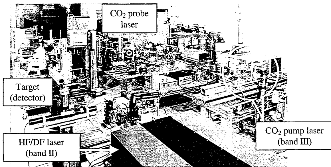
Figure 2. Experimental set-up
