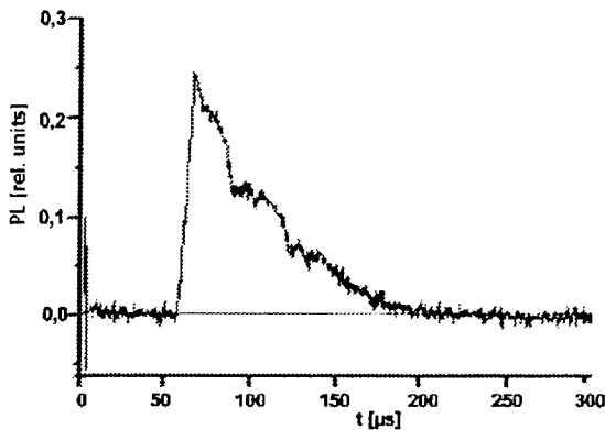
Fig. 7. Laser pulse form, laser energy 4.4 J
