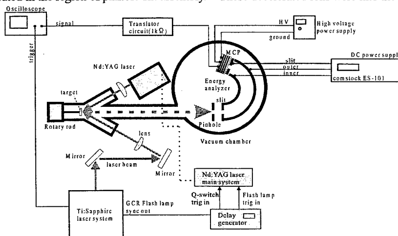
Fig.1 Experimental setup for TOF measurements using Ti:sapphire laser and Nd:YAG laser.
