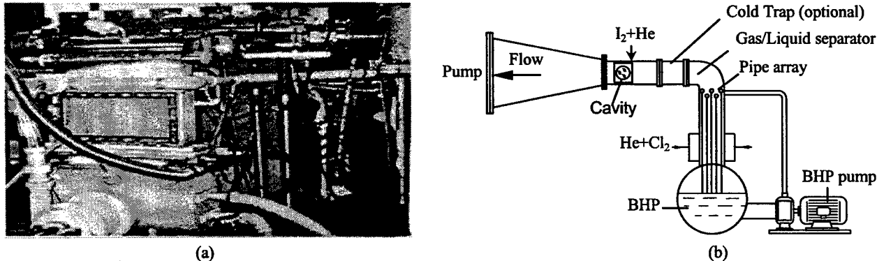
Fig.1 The experimental setup of COIL with a PJSOG
