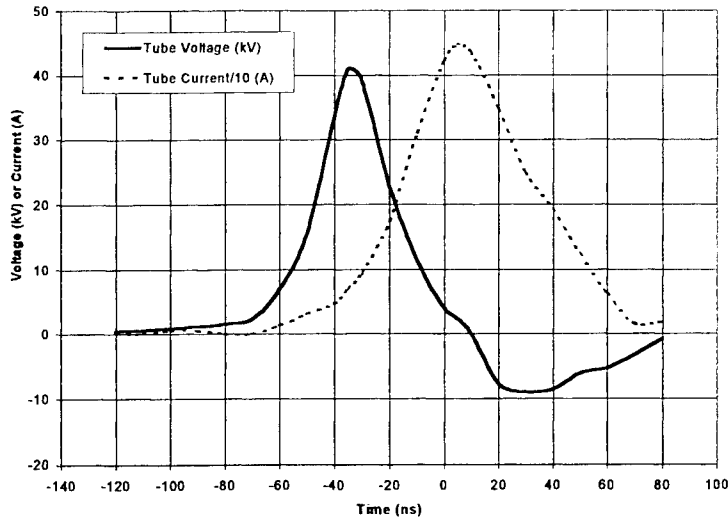
Fig. 5 : Electrical signals on the laser head.
