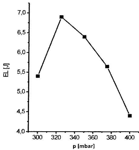
Fig. 5. Laser pulse energy vs. gas pressure, loading voltage 46 kV
