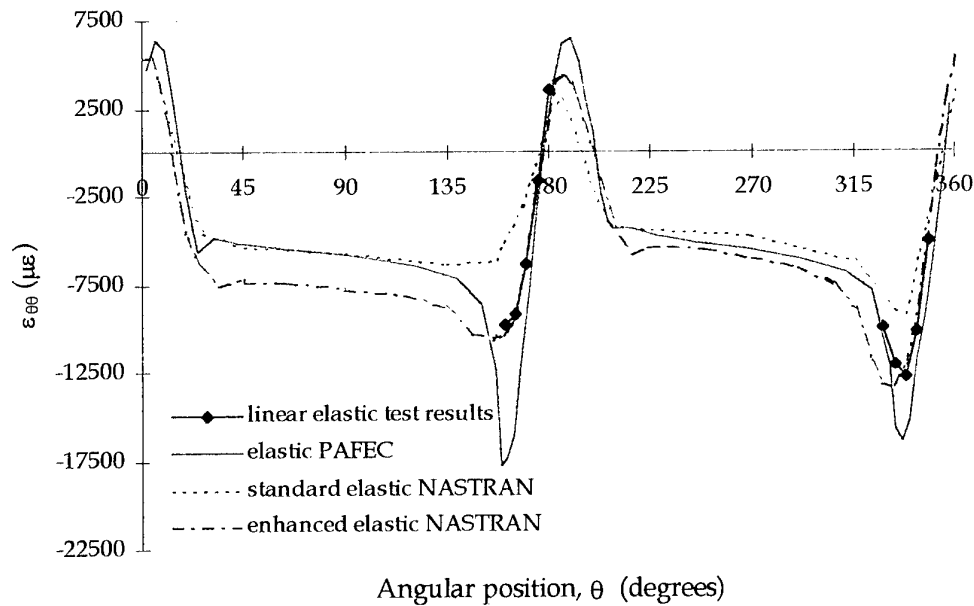
Figure 15: Comparison of hoop strain around FFWH #14 boundary at maximum CPLT load
