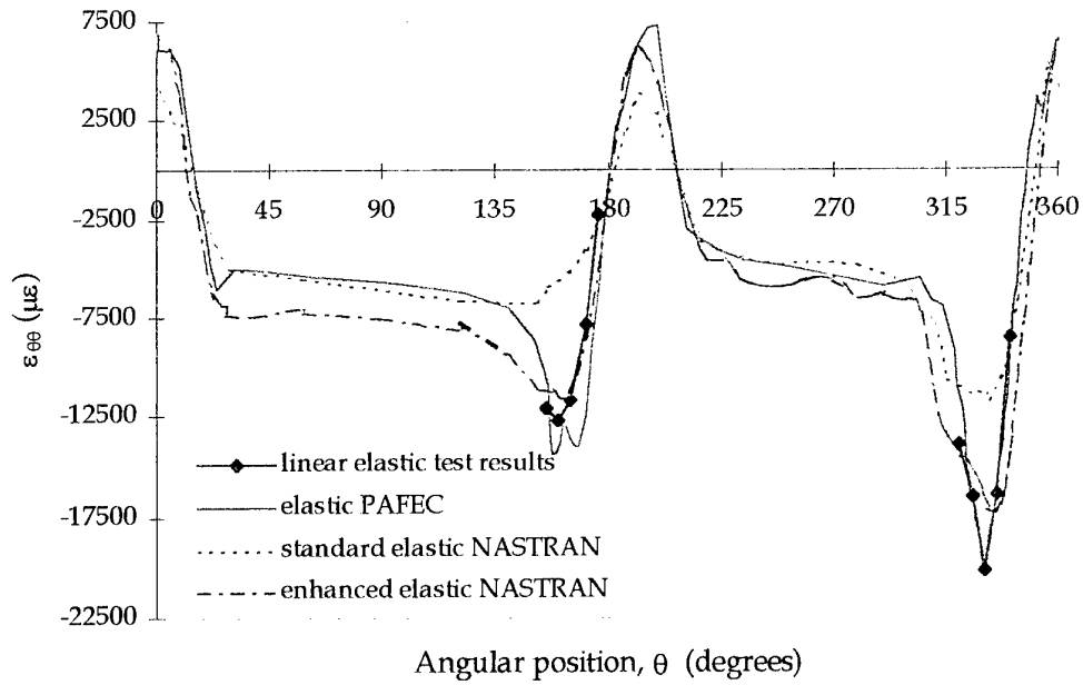
Figure 14: Comparison of hoop strain around FFWH #13 boundary at maximum CPLT load
