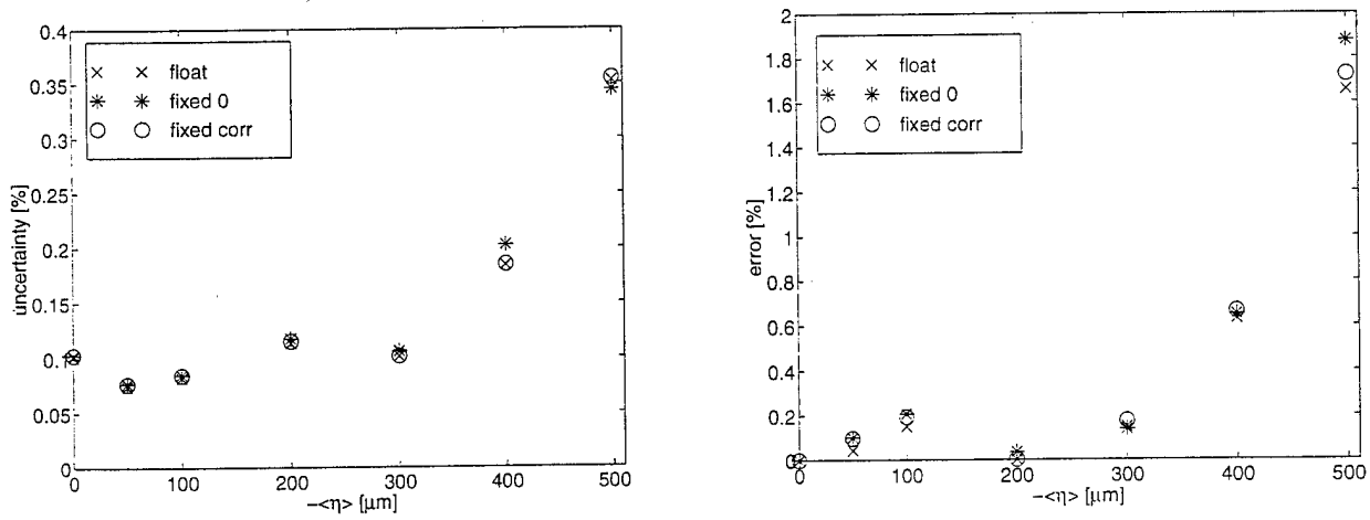
Figure 8: Uncertainty and error of sound speed vs. \bar{\eta} . The sound speed for \bar{\eta} = 0 is taken as reference. Three different fitting strategies were used. In the strategy denoted by “float,” \bar{\eta} is a floating fitting parameter, in “fixed 0,” \bar{\eta} is fixed at zero, and in “fixed corr,” \bar{\eta} was held constant at the correct preset value. The experimental conditions are the same as in Fig. 4.
