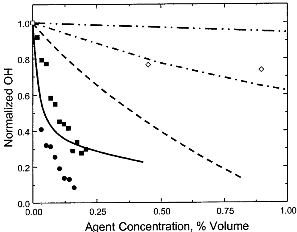
Figure 6. Normalized OH Concentrations vs. Delivered Inhibitor Agent Concentrations. The (●) Are the Experimental Fe(CO) 5 Data, and the Solid Line Is the Numerical Fe(CO) 5 Data; the (■) Are the Experimental DMMP Data, and the Dashed Line Is the Numerical DMMP Data; the (◇) Are the Experimental CF 3 Br Data, and the Dashed-Dot-Dashed Line Is the Numerical CF 3 Br Data. The Near Horizontal Dashed-Dot-Dot-Dashed Line Represents the N 2 Data Trend.
