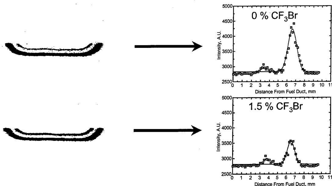
Figure 2. Representative PLIF Images and the Corresponding OH Intensity Profiles From an Opposed Flow Propane/Air Flame Seeded With 0% (by Volume) CF 3 Br and 1.5% (by Volume) CF 3 Br. Note: The Orientation of the PLIF Images With Respect to the Burner System Places the Fuel and Air Ducts at the Top and Bottom of Each Image, Respectively.
