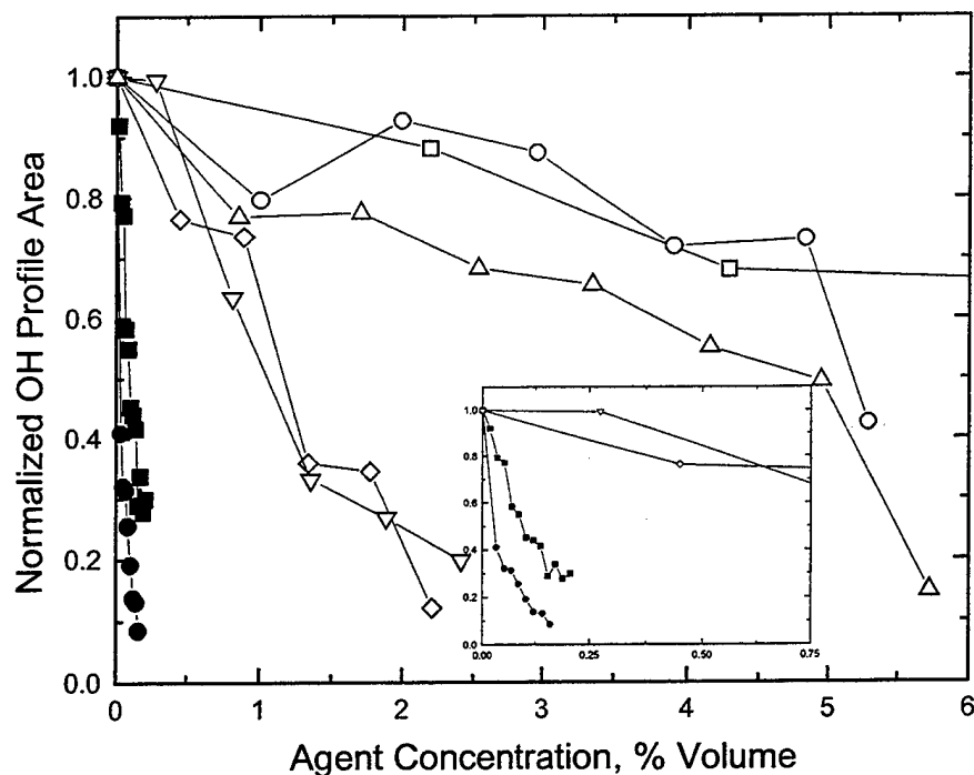
Figure 3. Normalized OH LIF Profile Areas vs. Inhibitor Agent Delivery Concentrations. The ( \square ) Are the N_2 Data, the ( \circ ) Are the FM-200 Data, the ( \Delta ) Are the FE 36 Data, the ( \nabla ) Are the PN Data, the ( \diamond ) Are the CF_3Br Data, the ( \blacksquare ) Are the DMMP Data, and the ( \bullet ) Are the Fe(CO)_5 Data. Inserted in the Figure Is a Second Plot of the PN, CF_3Br , DMMP, and Fe(CO)_5 Data for Agent Concentration up to 0.75% Volume.
