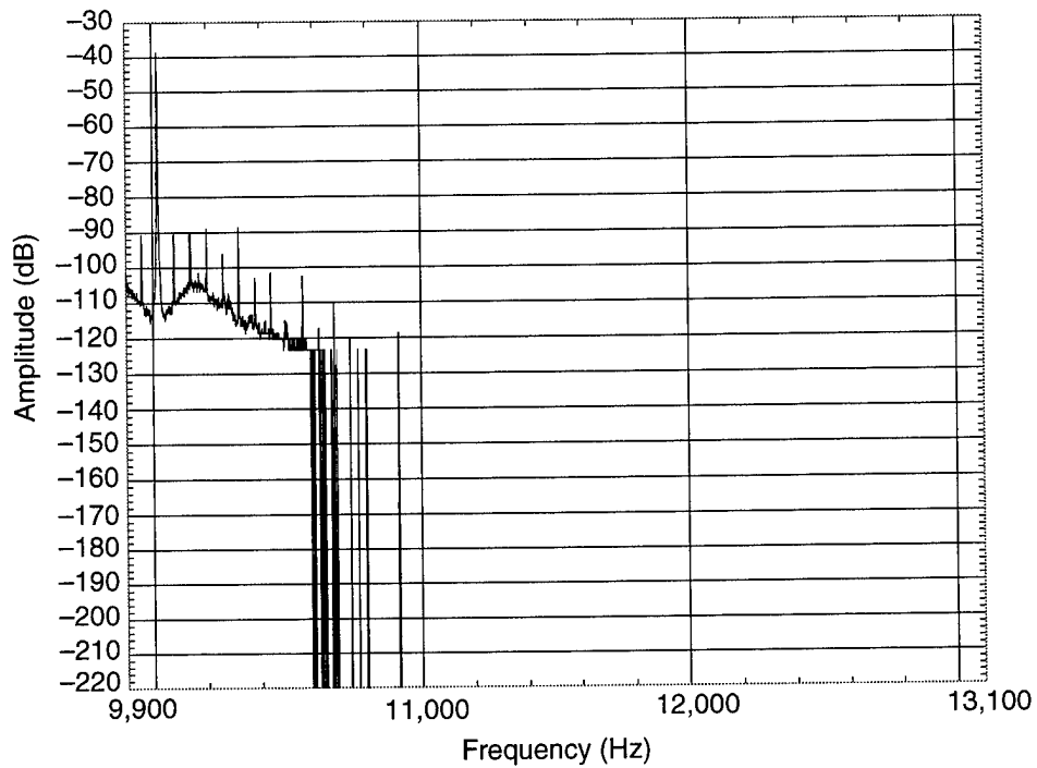
Figure C-112. Baseline measurement oscillator 74, screw sideways, vertical vibration.
