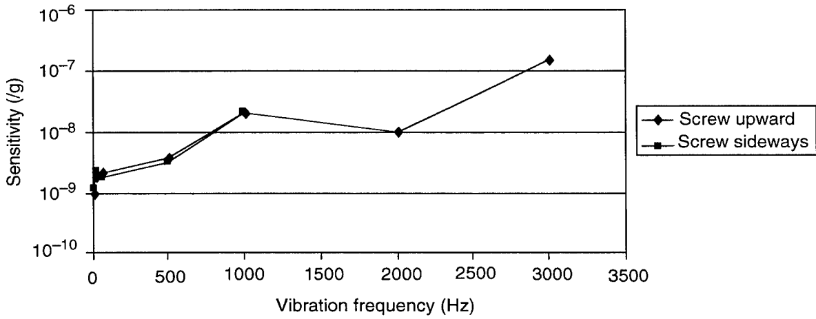
Figure 7. Average vibration sensitivity for device 716774.
