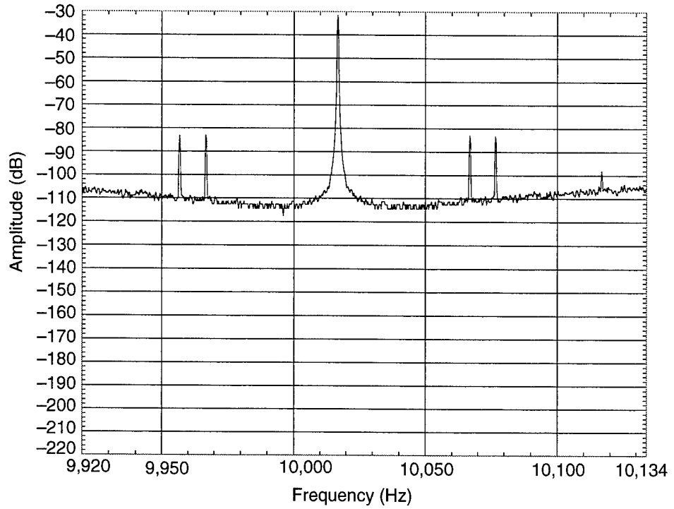
Figure C-121. Oscillator 74, 31.9 g at 50 Hz, screw sideways, vertical vibration, \gamma = 1.62 \times 10^{-9}/g .
