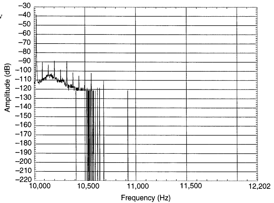
Figure C-18. Oscillator 96, 5 g at 2000 Hz, screw up, vertical vibration.
