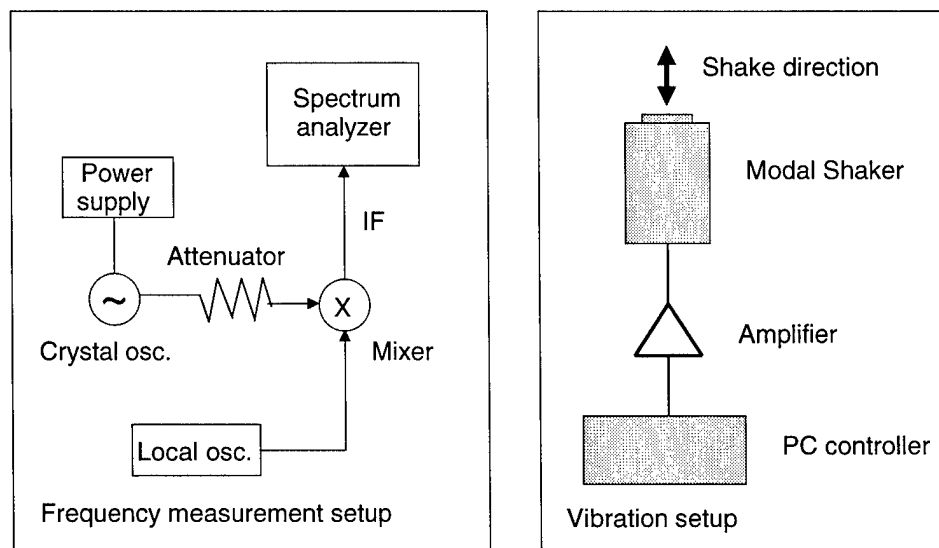
Figure 1. Experimental test setup
