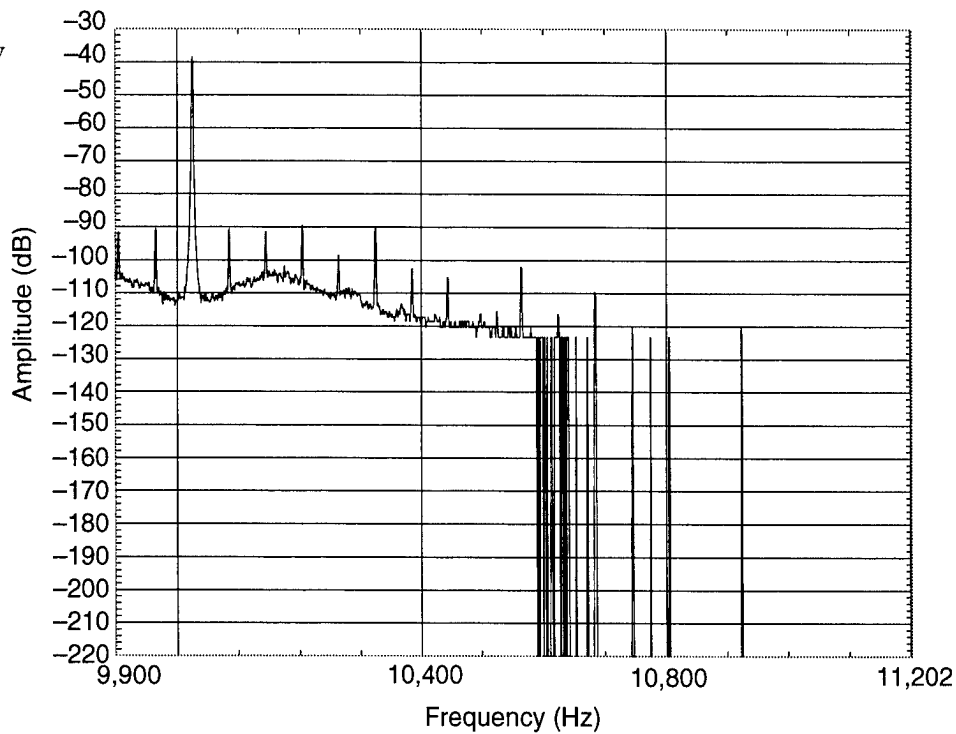
Figure C-42. Oscillator 96, 1 g at 1000 Hz, screw sideways, vertical vibration, can't resolve.
