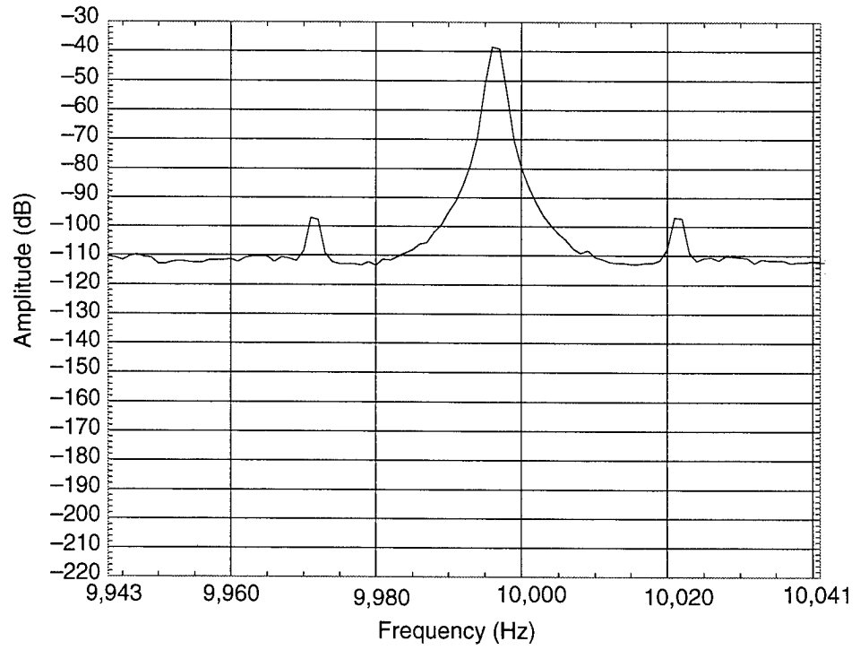
Figure C-89. Oscillator 74, 8 g at 25 Hz, screw up, vertical vibration, \gamma = 1.40 \times 10^{-9}/g .
