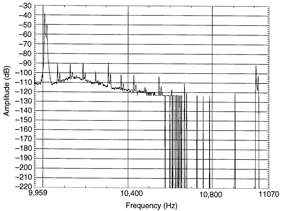
Figure C-130. Oscillator 74, 25 g at 1000 Hz, screw sideways, vertical vibration, \gamma = 4.02 \times 10^{-8}/g .
