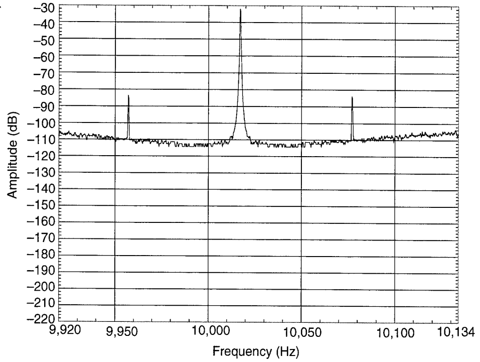
Figure C-117. Oscillator 74, 1 g at 50 Hz, screw sideways, vertical vibration, No Signal.
