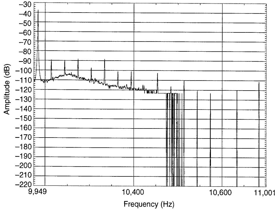
Figure C-129. Oscillator 74, 10 g at 1000 Hz, screw sideways, vertical vibration, \gamma = 7.98 \times 10^{-9}/g .
