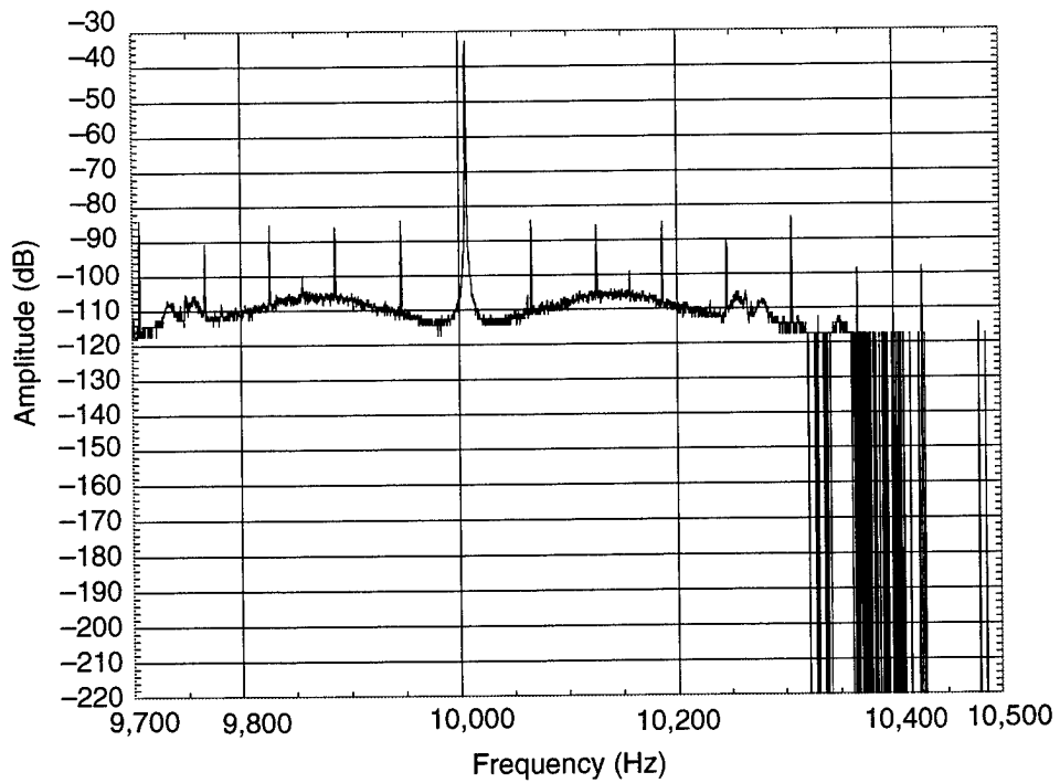
Figure C-56. Baseline measurement oscillator 96, device horizontal, vertical vibration.
