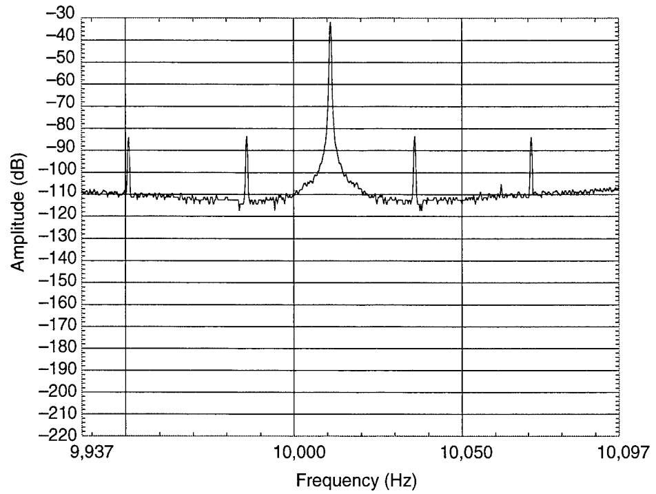
Figure C-29. Oscillator 96, 5 g at 25 Hz, screw sideways, vertical vibration, \gamma = 5.63 \times 10^{-9}/g .
