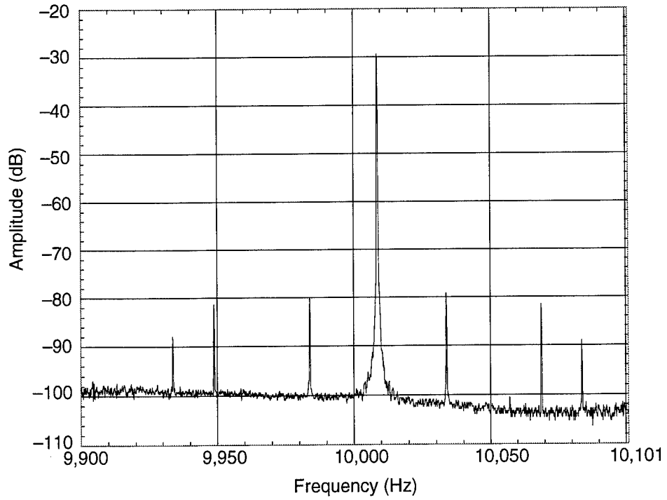
Figure C-3. Oscillator 96, 5 g at 25 Hz, screw up, vertical vibration, \gamma = 6.47 \times 10^{-9}/g .
