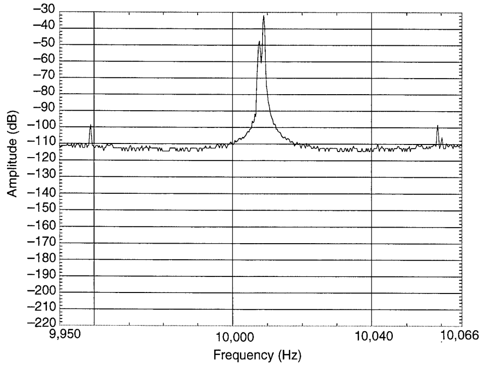
Figure C-61. Oscillator 96, 1 g at 50 Hz, device horizontal, vertical vibration, \gamma = 8.93 \times 10^{-9}/g .
