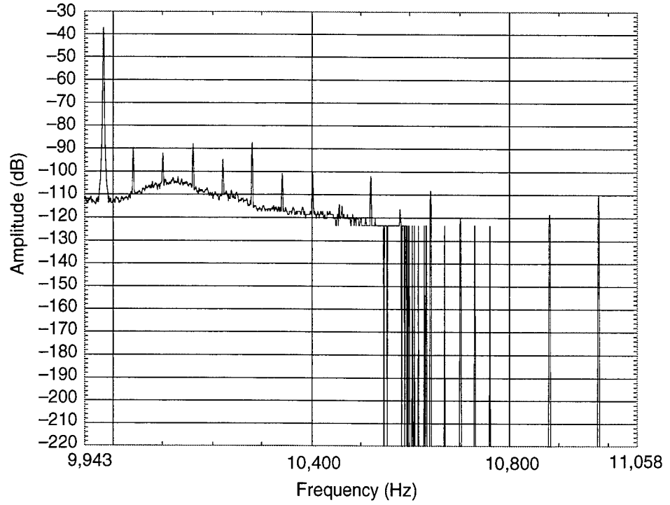
Figure C-101. Oscillator 74, 10 g at 1000 Hz, screw up, vertical vibration, \gamma = 8.95 \times 10^{-9}/g .
