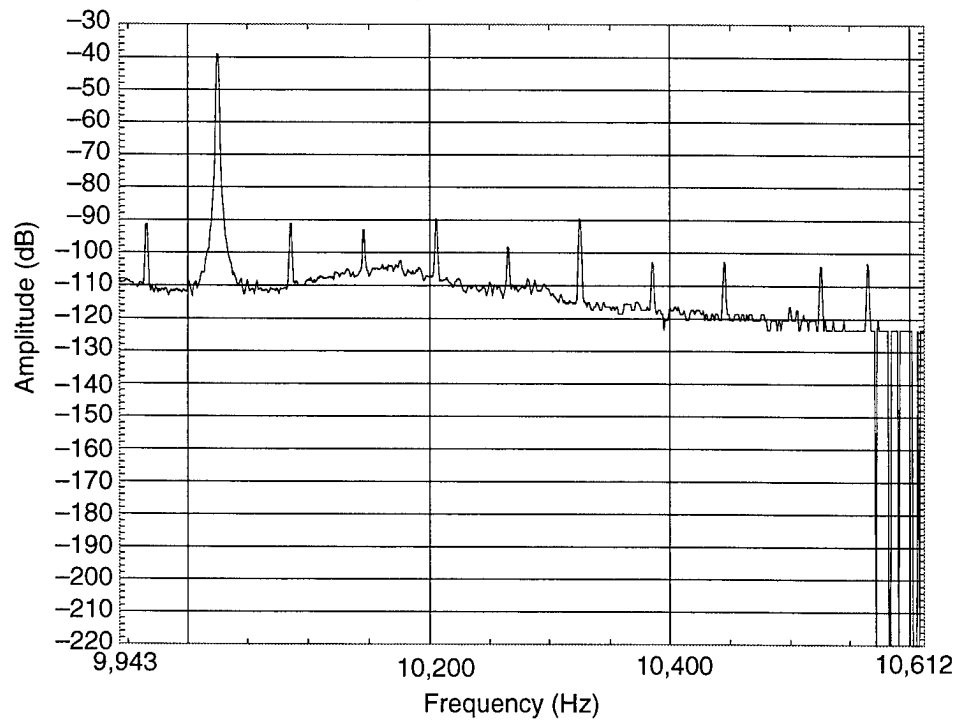
Figure C-70. Oscillator 96, 25 g at 500 Hz, device horizontal, vertical vibration, \gamma = 4.50 \times 10^{-9}/g .
