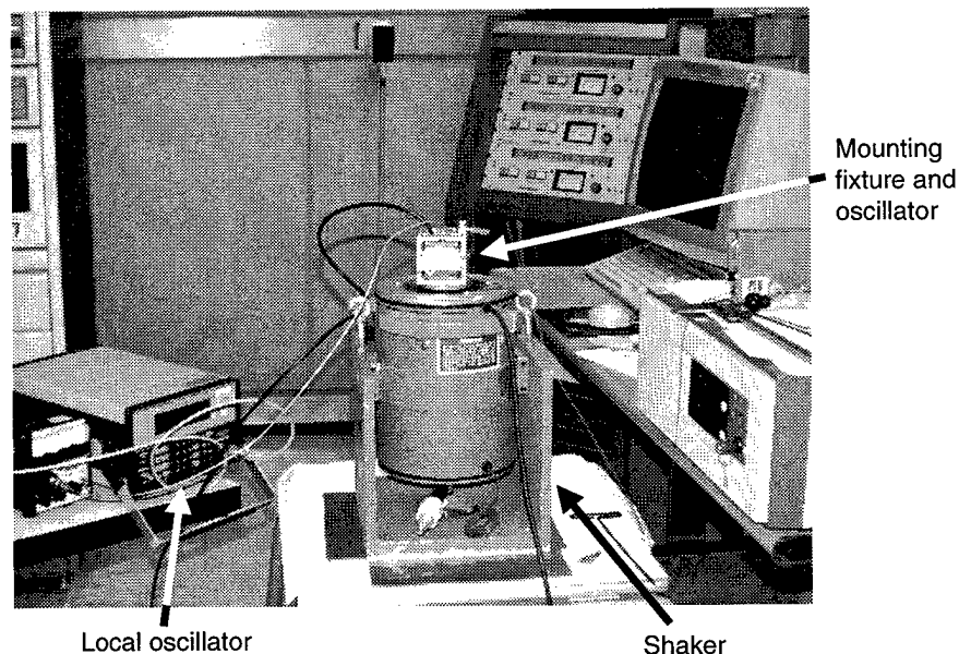
Figure 2. Shaker, mounting fixture, and oscillator.
