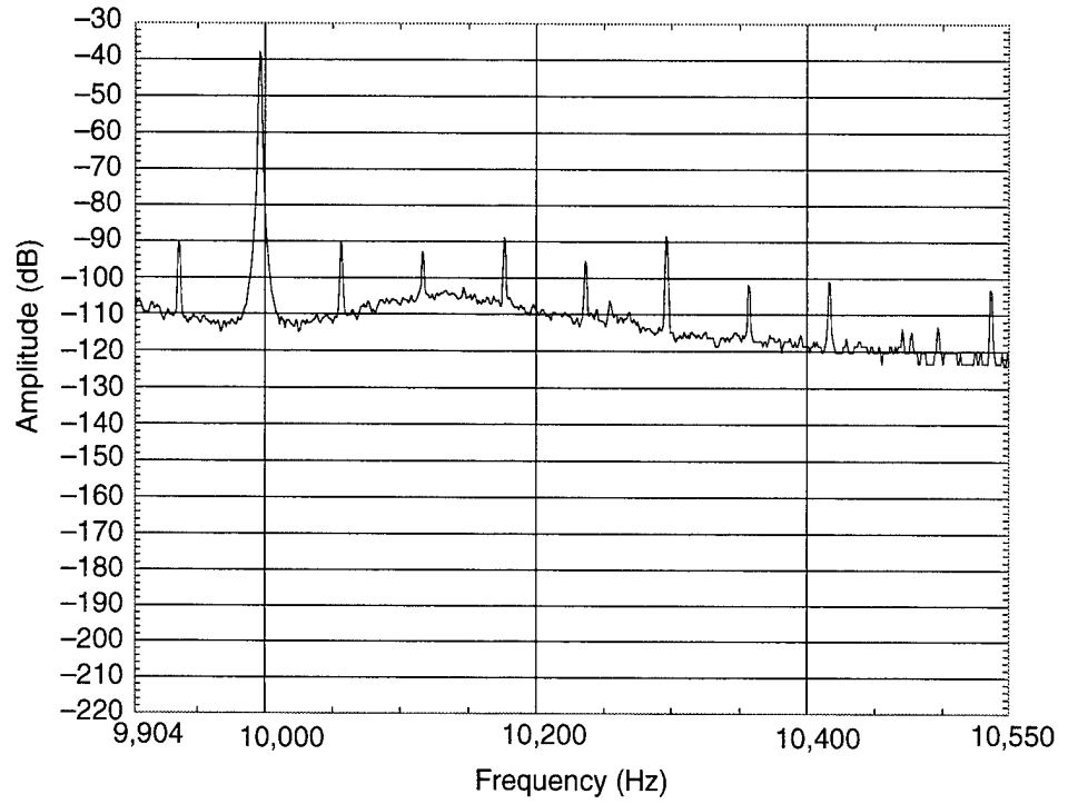
Figure C-97. Oscillator 74, 10 g at 500 Hz, screw up, vertical vibration, \gamma = 3.56 \times 10^{-9}/g .
