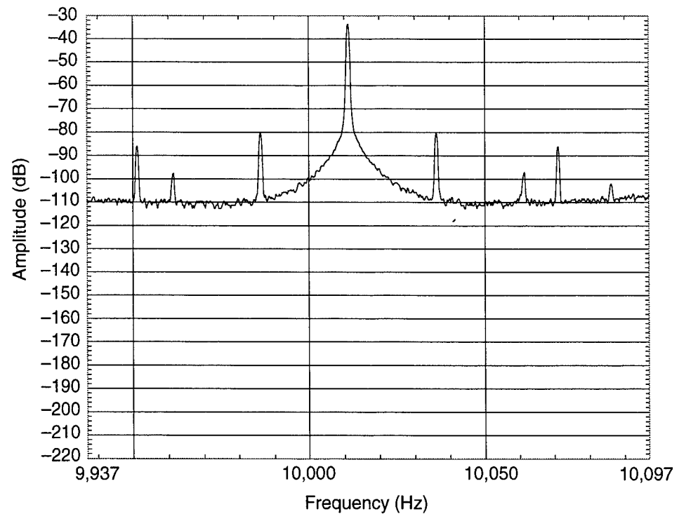
Figure C-30. Oscillator 96, 8 g at 25 Hz, screw sideways, vertical vibration, \gamma = 5.58 \times 10^{-9}/g .
