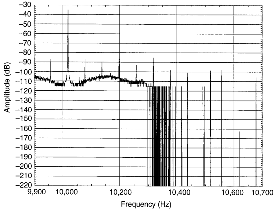
Figure C-9. Oscillator 96, 9 g at 500 Hz, screw up, vertical vibration, \gamma = 1.57 \times 10^{-8}/g .
