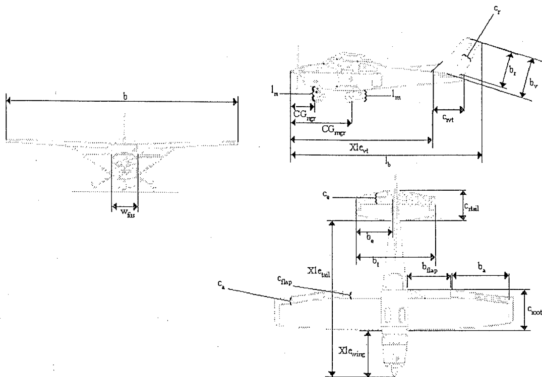
Figure 2.1. Definition of Design Variables
