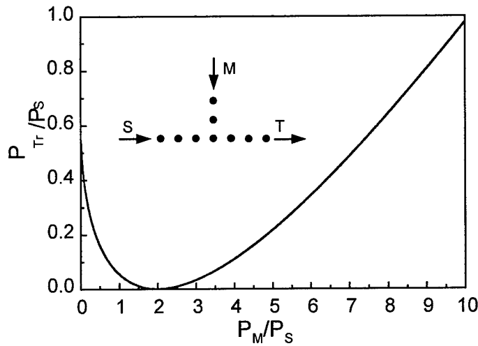
Figure 3. Dependence of the normalized transmitted power, P_{Tr}/P_S , as a function of the normalized modulation power, P_M/P_S of the switch depicted in the inset. The switch consists of two orthogonal chains of metal nanoparticles. The specific functional dependence is valid for the case that the signal plasmon wave, S, and transmitted plasmon wave, T, are longitudinal and the modulation plasmon wave is transverse and out of phase with S.
