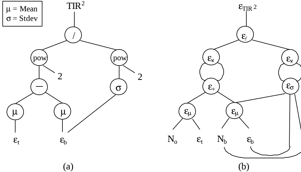
Figure 4. Error function of the ADGF (a) Algorithm dataflow graph, and (b) Error function dataflow graph. The results are \text{TIR}^2 and \epsilon_{\text{TIR}^2} .
