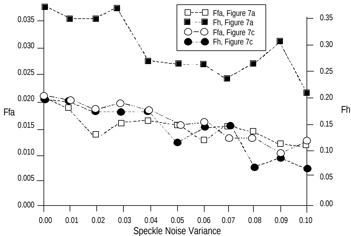
Figure 10. Fh and Ffa as a function of speckle noise variance ranging from 0.0 to 0.1, where (H,W,e) = (11,8,5) , and images from Figures 7a and 7c are employed.
