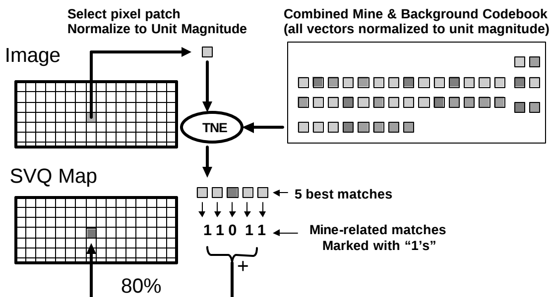
Figure 13: Notional diagram of the SVQ process.
