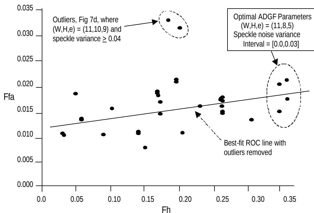
Figure 8. ROC curve of all ADGF test cases where F_h > 0 , from Tables 6 and 8.
