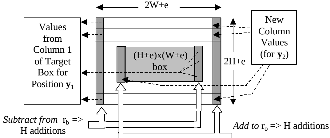
Figure 3. Buffering scheme for efficient computation of background mean r_b , if H \leq W .
