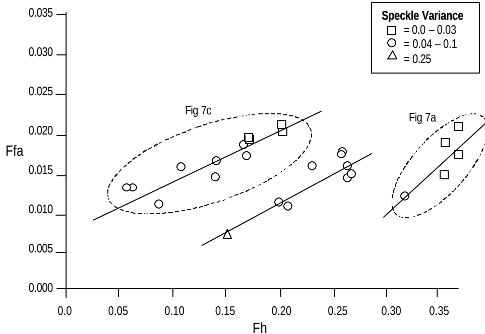
Figure 9. ROC plot of F_{fa} versus F_h for (W,H,e) = (11,8,5) .
