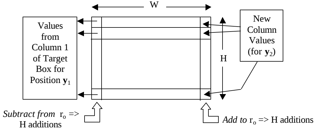
Figure 2. Buffering scheme for efficient computation of target mean r_o , if H \leq W .
