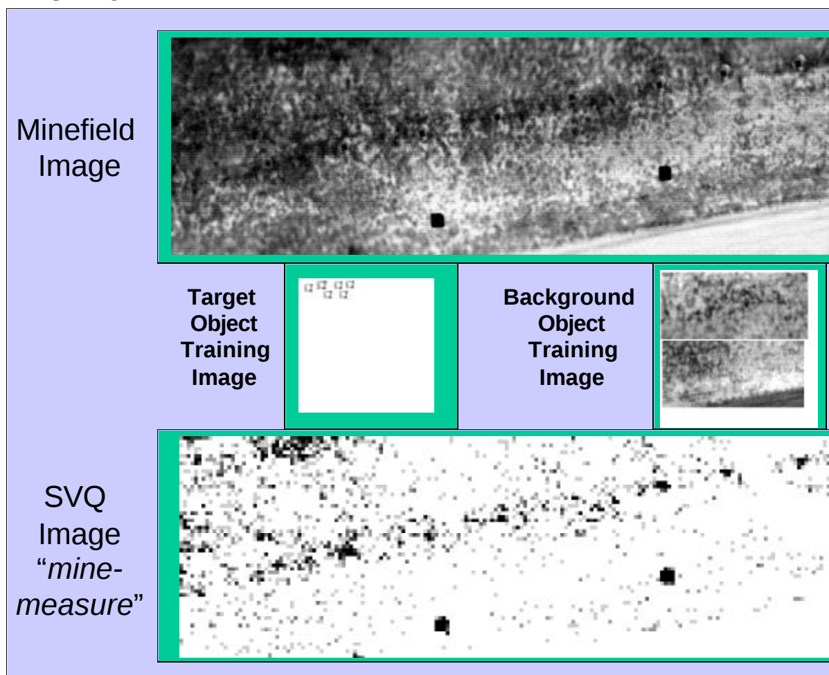
Figure 14. Example of SVQ applied to a minefield image. Note that in addition to the mines themselves, the procedure also highlights the adjacent regions. This results from training on the surrounding regions.
