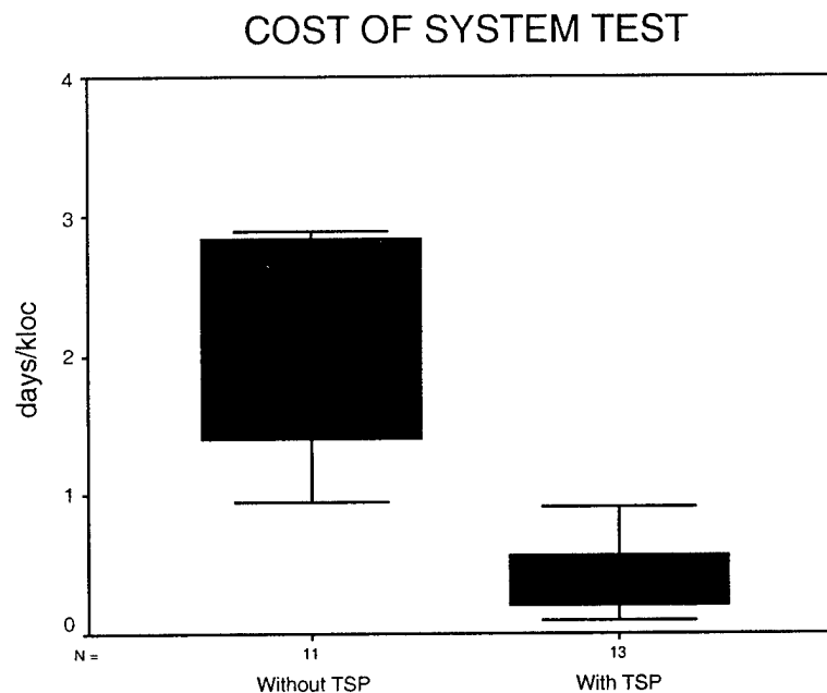
Figure 14: Reductions in Test Duration
