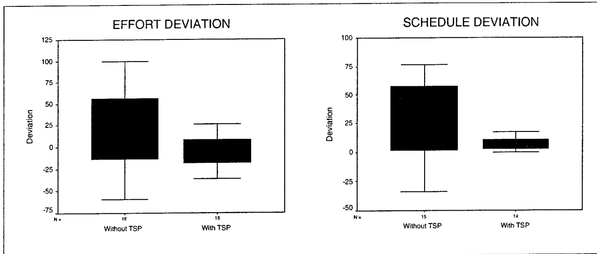
Figure 11: Effort and Schedule Deviation
