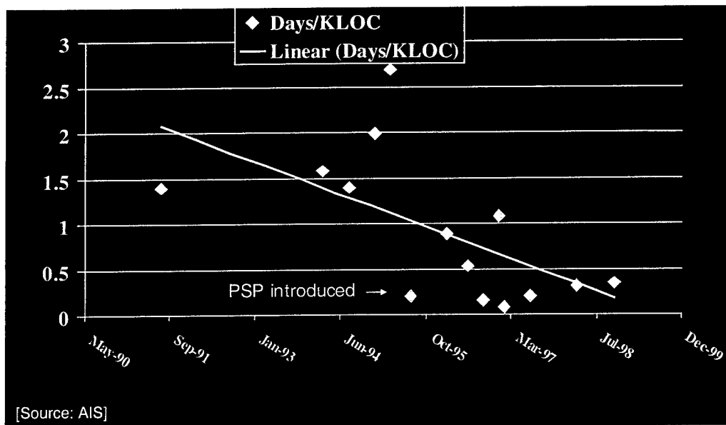
Figure 9: AIS System Test Duration
