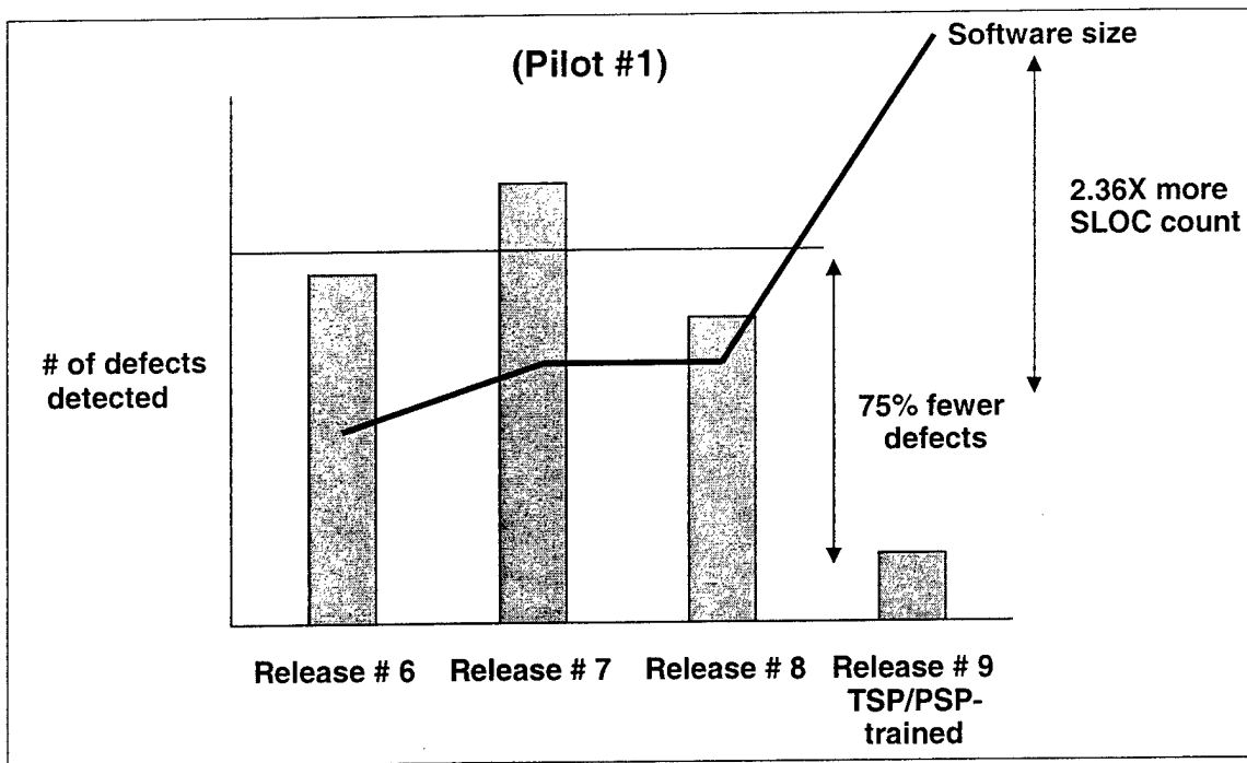
Figure 4: Boeing Defect Data for Pilot 1
