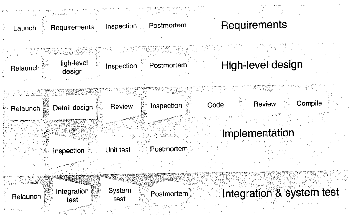
Figure 1: The TSP Structure
