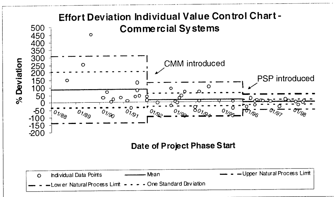
Figure 6: AIS Effort Deviation
