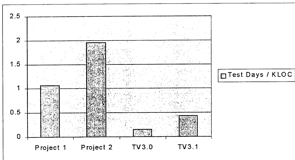
Figure 3: Hill AFB Test Duration
