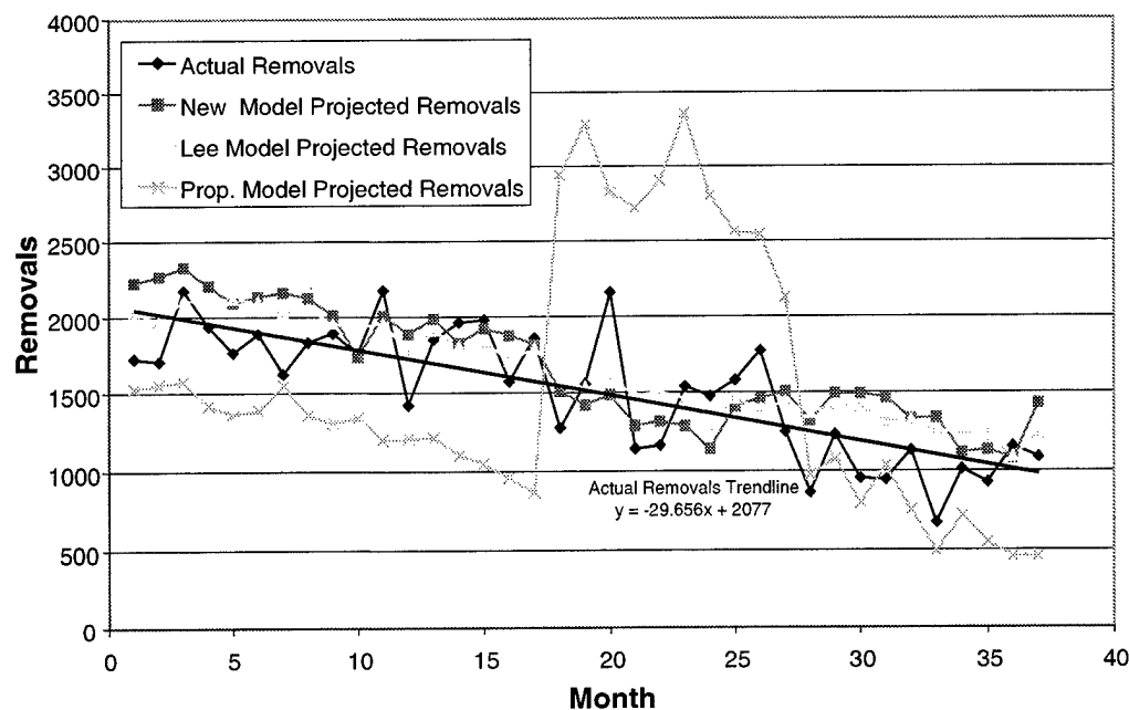
Figure 4-5. Fit of Models to C-5B Data After Treating Bathtub Trend (calibration period: months 10–21)
