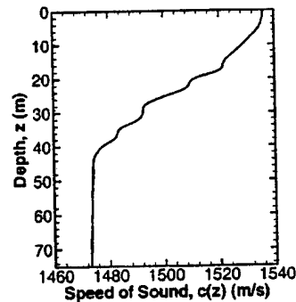
FIG. 2. Speed of sound versus depth for the standard sound channel. This profile is based on measurements made during the 1995 SWARM experiment and was provided to the authors by Dr. Steven Finette of the Naval Research Laboratory.
