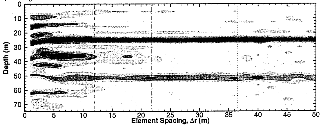
(c) Endfire TRA
