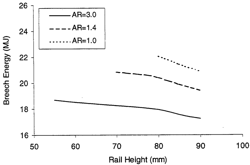
Figure 6. Breach Energy as a Function of Rail Height.
