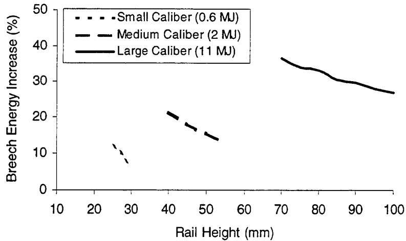
Figure A-3. Increase in Breach Energy for an Augmented Launcher ( V_f=2500 m/s).
