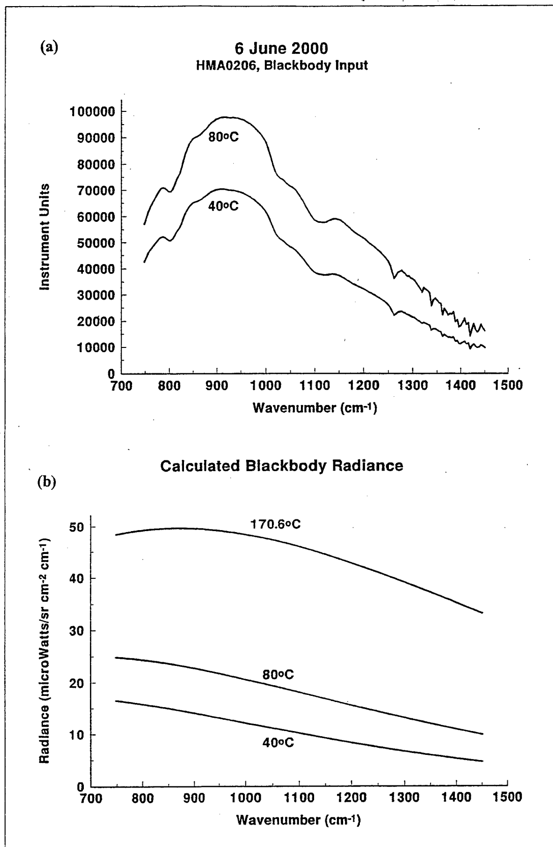
Figure 7. Calculation of responsivity/self-emission terms requires (a) single-beam response to (b) blackbody radiance level
