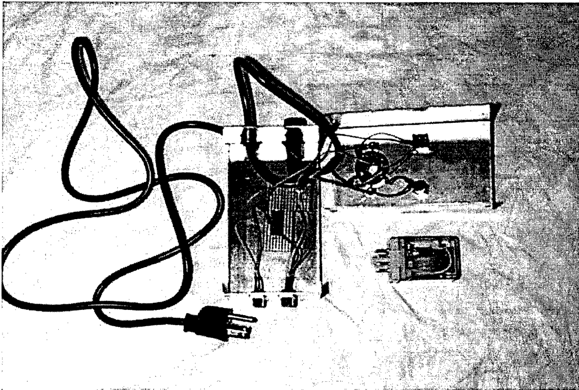
Commercial Power Interface: Internal w/ IDEC RR2PU-120VAC Relay
