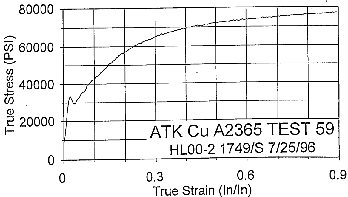
Fig. 18b Hopkinson bar compression stress-strain data from test 59 obtained on a longitudinal specimen from the ATK plate at the orientation of 0^\circ at the strain rate of 1749/s.
