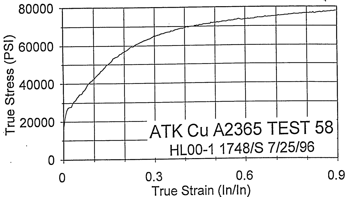
Fig. 18a Hopkinson bar compression stress-strain data from test 58 obtained on a longitudinal specimen from the ATK plate at the orientation of 0^\circ at the strain rate of 1748/s.
