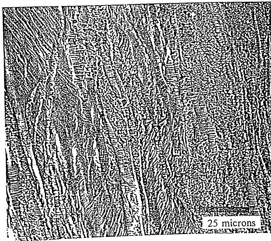
Fig. 10 An optical micrograph of copper showing deformation banding.
