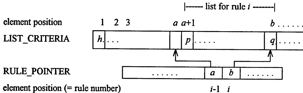
Figure 2. Data structure for rule base.
