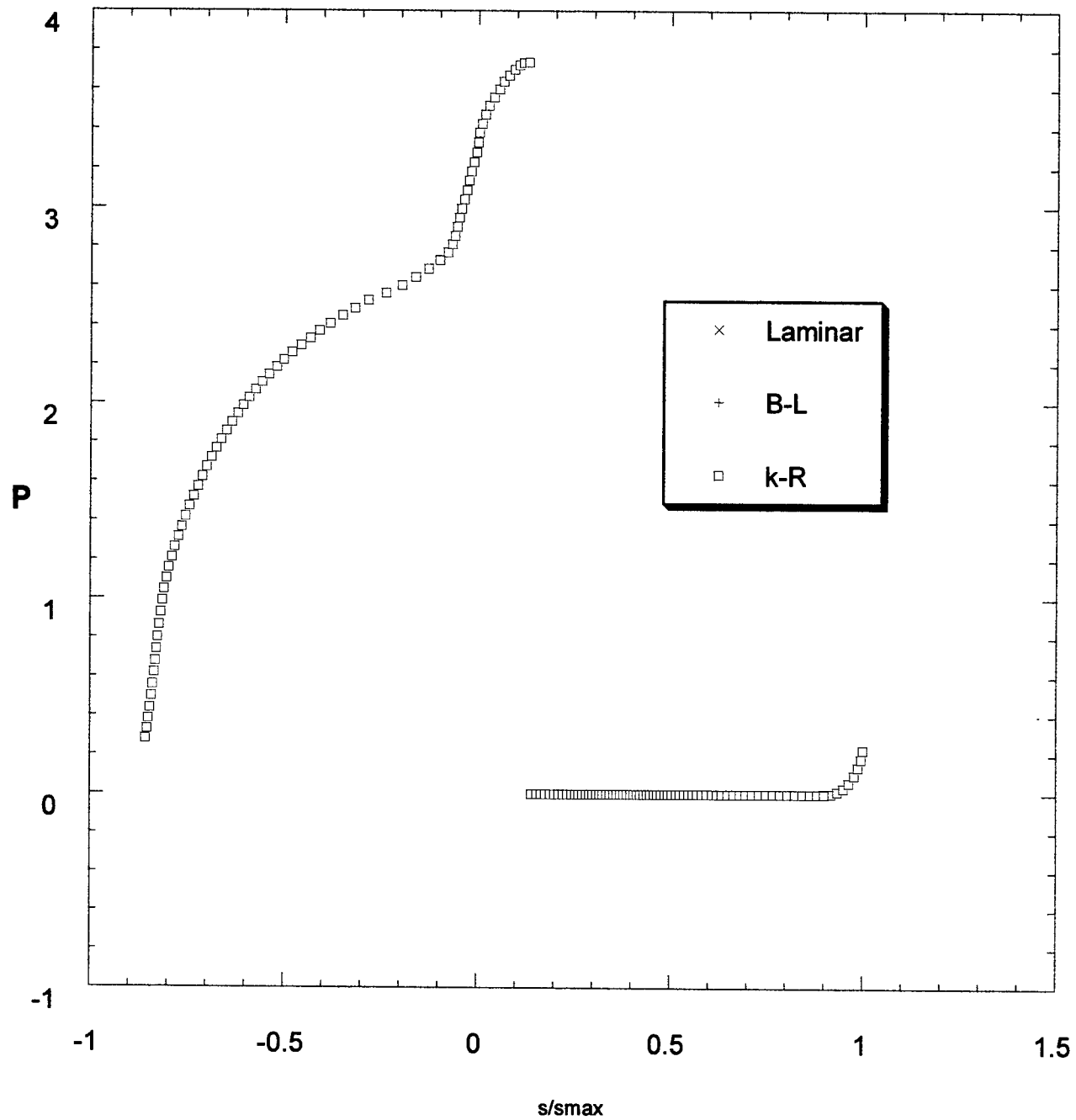
Figure 3. Dimensionless Pressure
