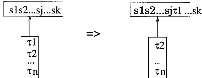
Figure 5: Job sequencing procedure.
