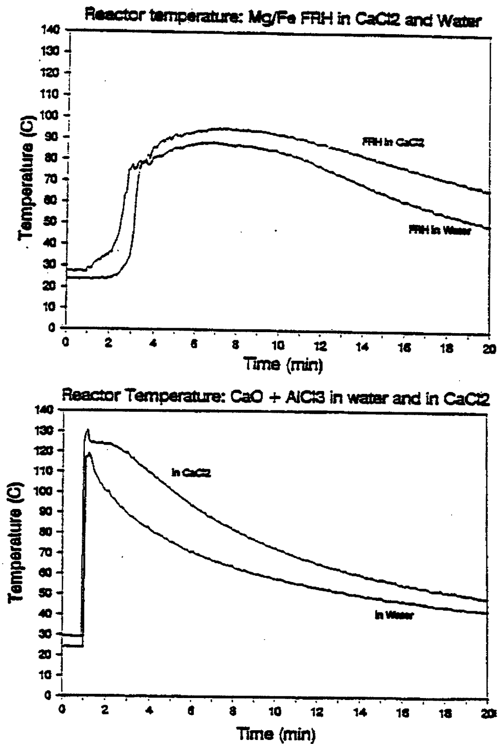
Figure 6, Comparison of reaction temperatures with water and with calcium chloride solution
