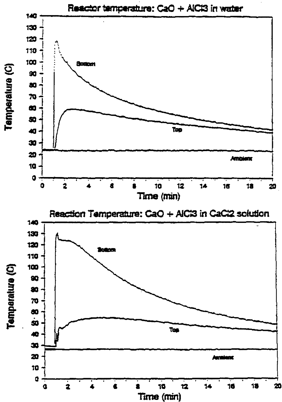
Figure 5, Reaction of aluminum chloride and calcium oxide with water and with calcium-chloride solution
