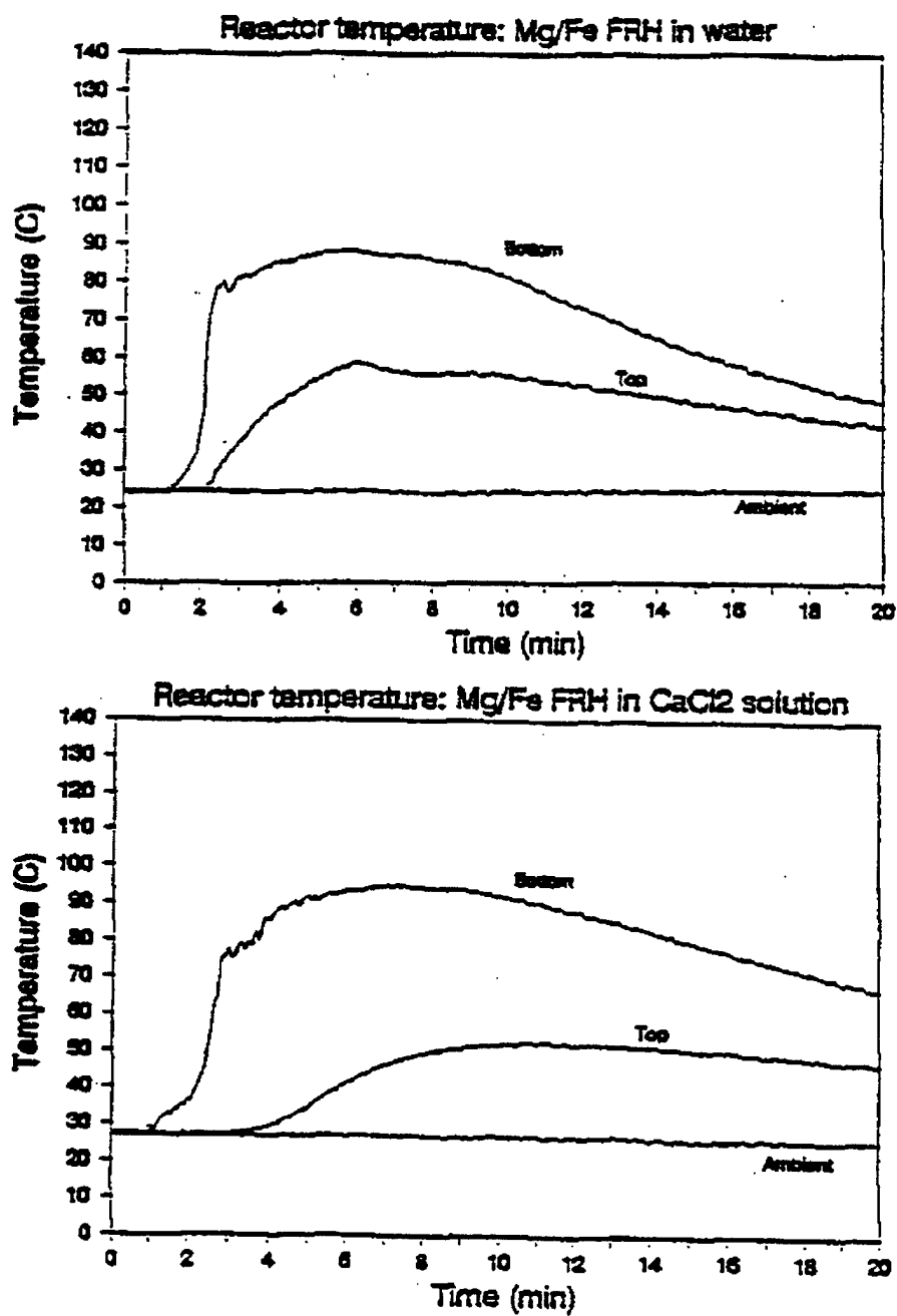
Figure 4, Reaction of Mg/Fe FRH with water and with calcium chloride solution
