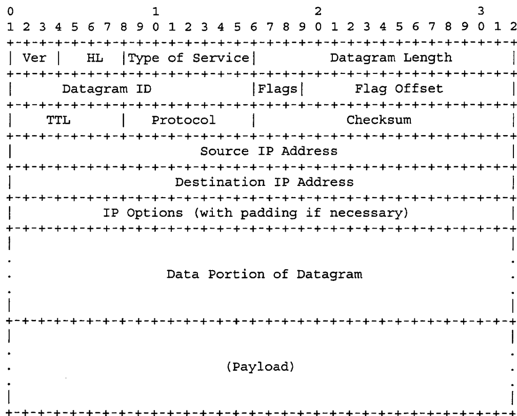
Figure 3-1 IPv4 Datagram Packet Header Format
