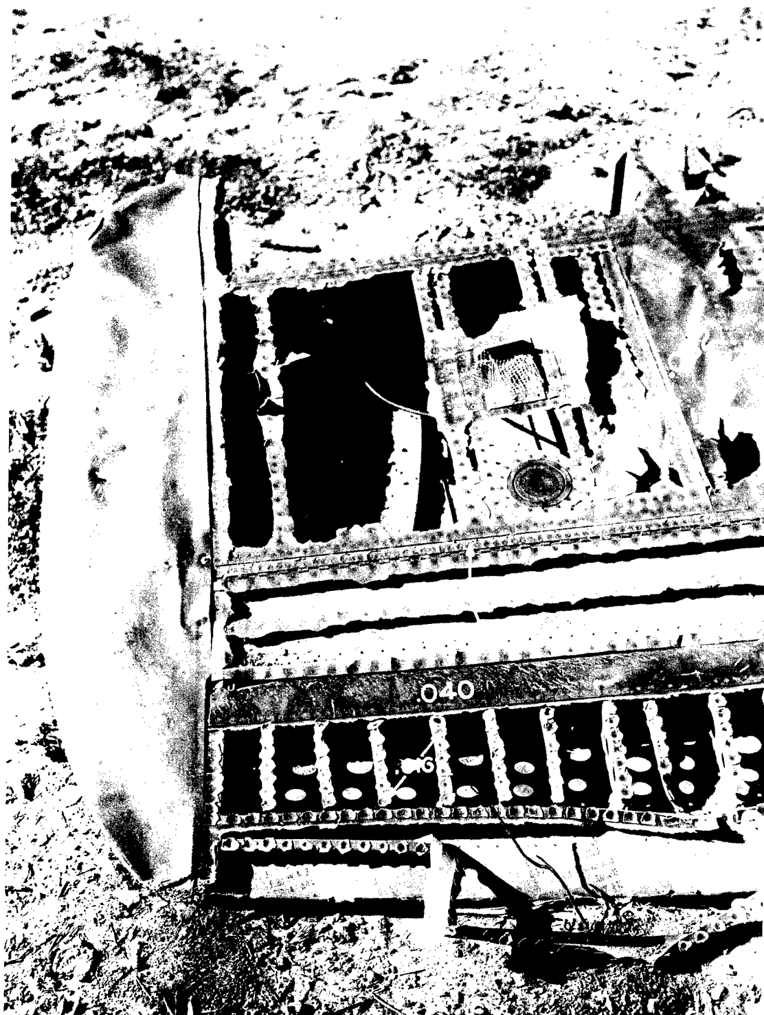
Fig. 2.16 AD-2, Outboard Port Wing Panel and Wing Tip Showing Wing Tip Intact. Note how white star protected 0.032 skin. - Shot 7
