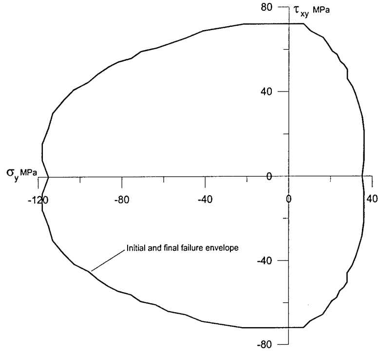
Fig. 4 Failure envelope for a [0°] lamina made from E-glass/LY556/HT907/DY063 under biaxial, \sigma_y/\tau_{xy} , load.
