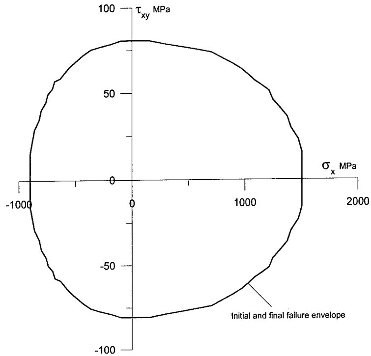
Fig. 5 Failure envelope for a [0°] lamina made from T300/BSL914C under biaxial, \sigma_x/\tau_{xy} , load.
