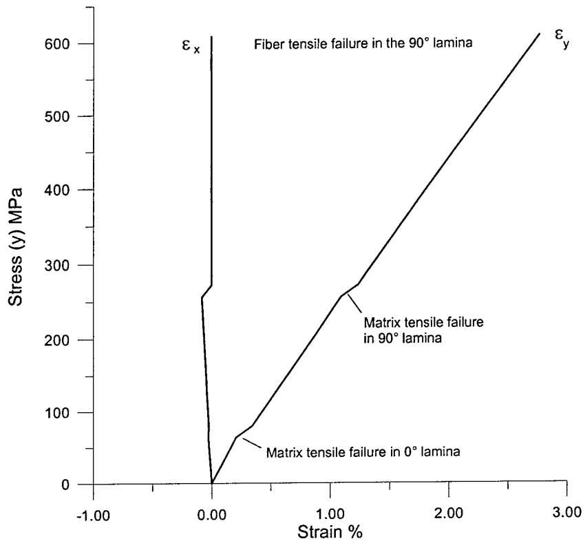
Fig. 15 Stress/strain curves for a [0°/90°/0°] laminate made from E-glass/MY750/HT917/DY063 under uniaxial tension load \sigma_y/\sigma_x = 1/0 .
