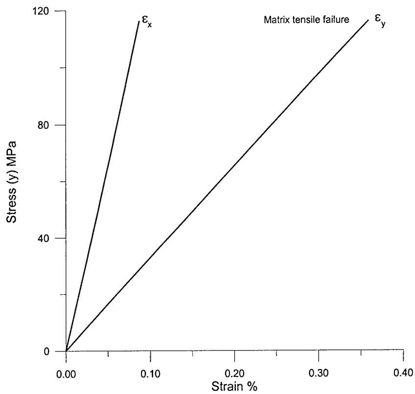
Fig. 14 Stress/strain curves for a [\pm 55]_s laminate made from E-glass/MY750/HT917 /DY063 under uniaxial tension load \sigma_y/\sigma_x = 2/1 .
