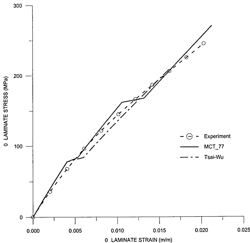
Figure 3. E-glass/vinylester [0/90/±45] s laminate under uniaxial tension.
