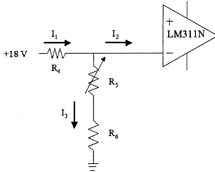
Figure 6.5: Voltage Divider Circuit [from 5].
