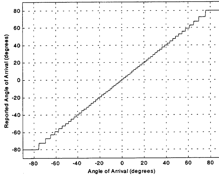
Figure 8.3: Ideal Transfer Function.
