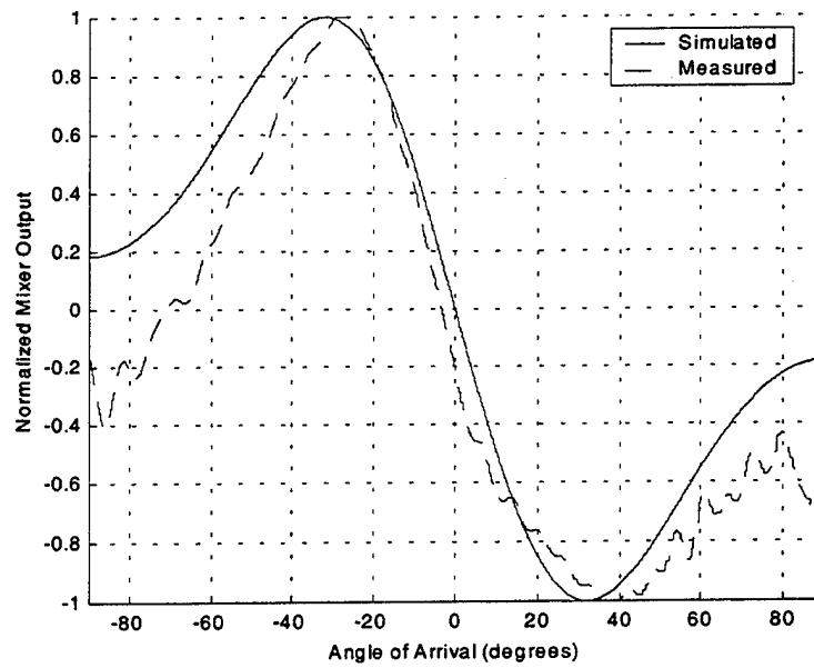
Figure 4.8: Normalized Mixer Output and Simulation Waveforms for RSNS Array with m_r=17 [from 5].
