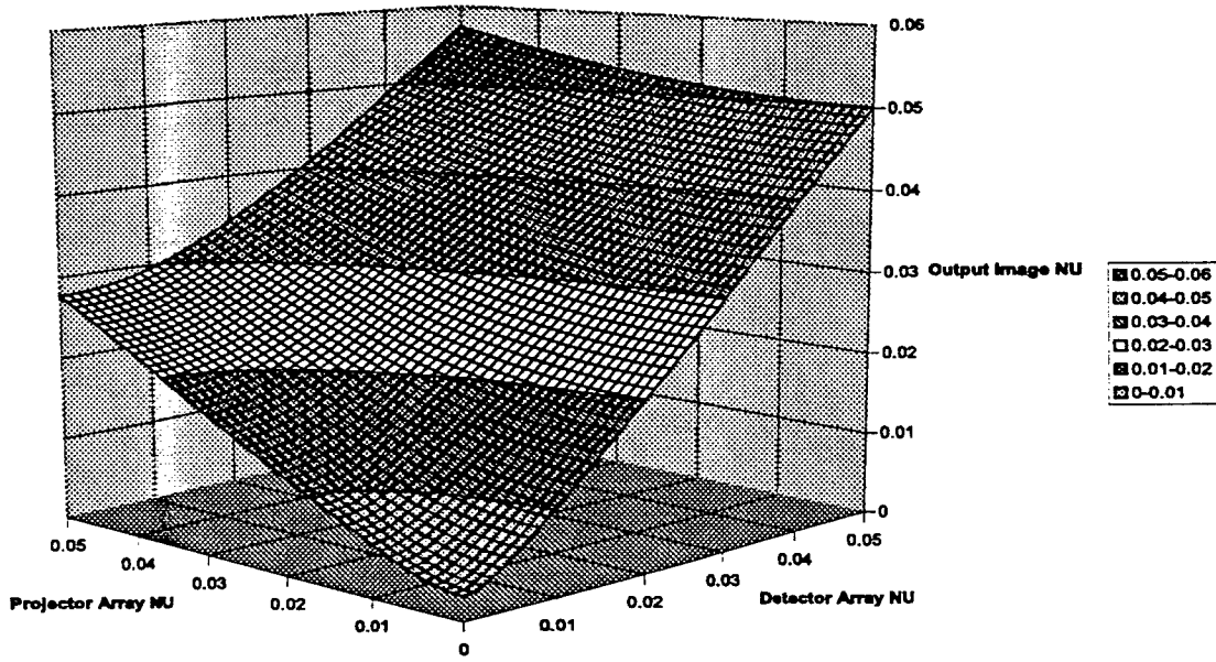
Figure 11: Output NU versus Detector NU and Projector NU with n/m = 1.04 , K = 1.5 , T_x = T_y = 0.0 , and F_x = F_y = 1 .
