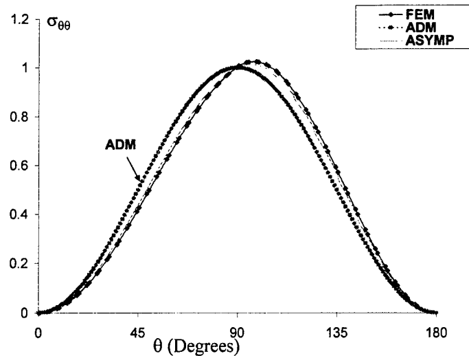
Figure 21: Opening stress angular variation comparison for problem - A
