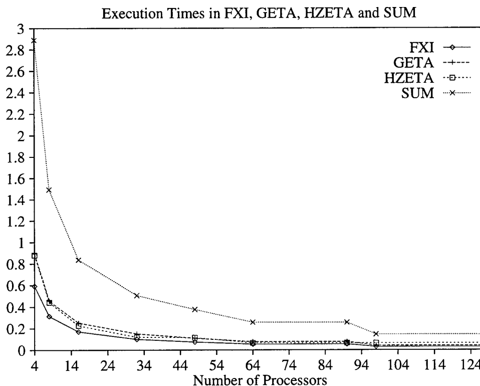
Figure 1: Execution Times of the Major Subroutines.
