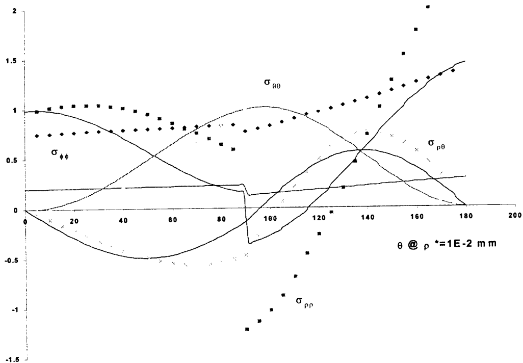
Figure 11: Angular variation matching with ADM solution at \rho^*=1E-2 \text{ mm}
