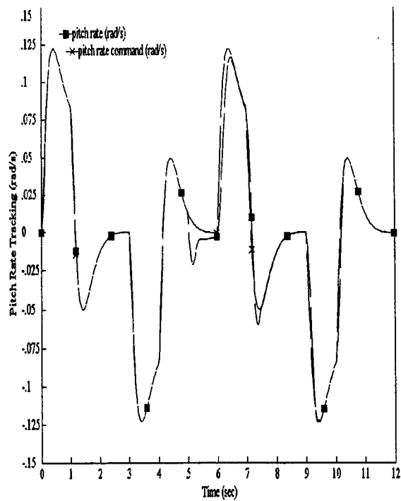
Fig. 18 Pitch rate tracking
