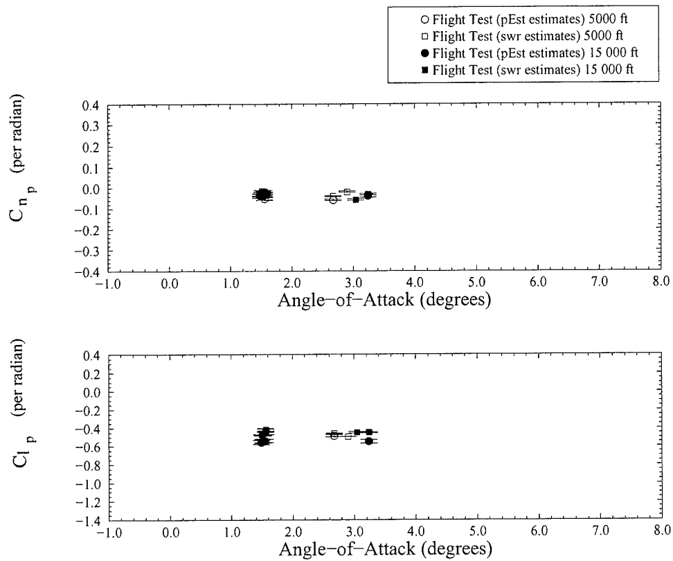
Figure 15: PC 9/A roll rate derivatives, take-off flap.
