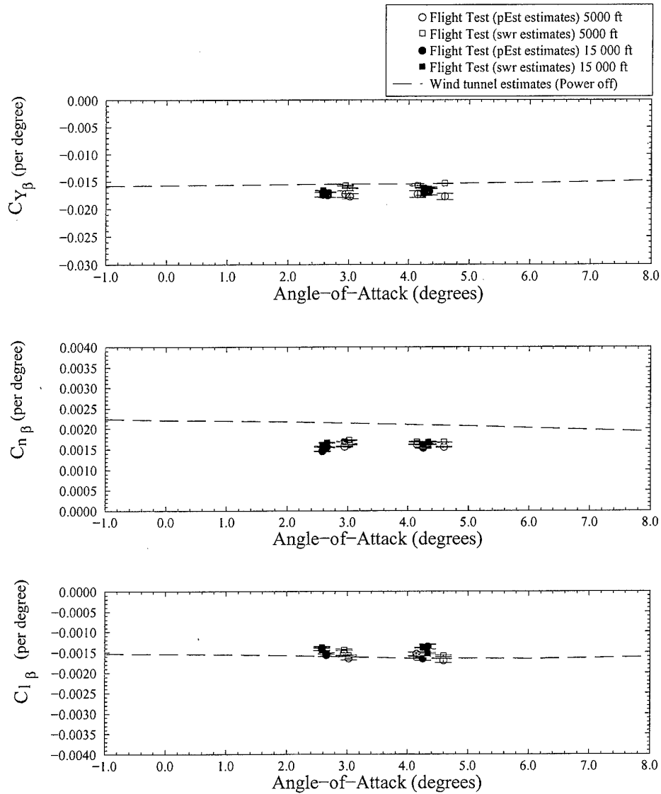
Figure 8: PC 9/A angle-of-sideslip derivatives, gear down.
