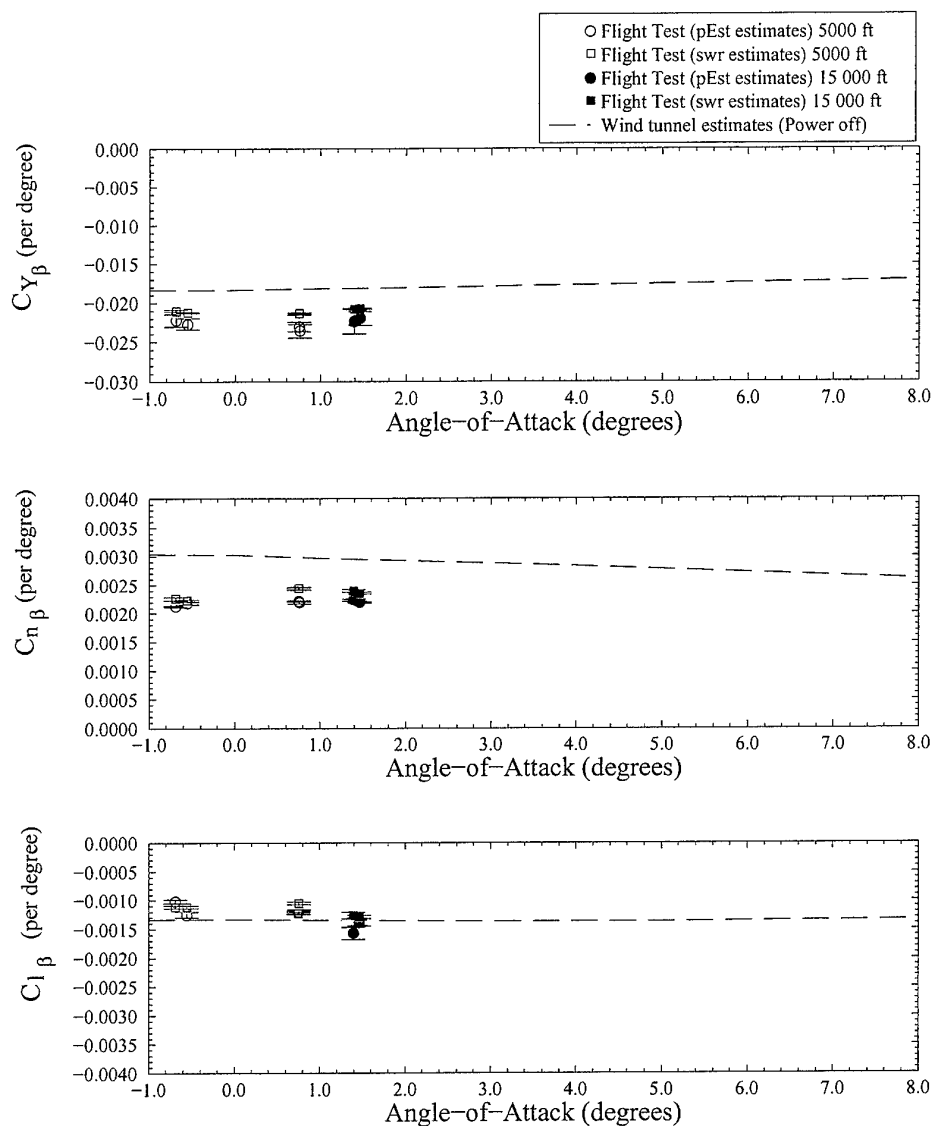
Figure 10: PC 9/A angle-of-sideslip derivatives, landing flap.
