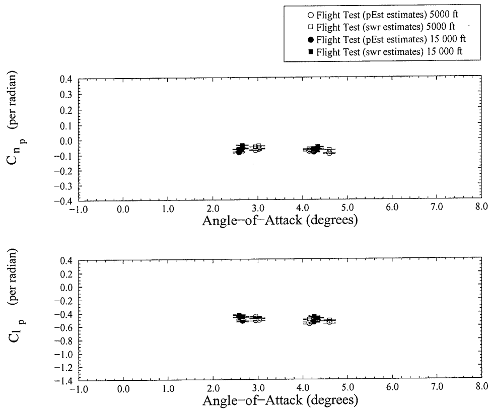
Figure 14: PC 9/A roll rate derivatives, gear down.
