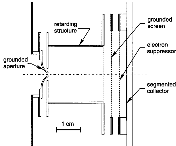
Figure 11. Cross-sectional view of the flowing plasma probe developed to analyze the density, flow velocity, and parallel and perpendicular ion temperatures in the flowing plasma.
