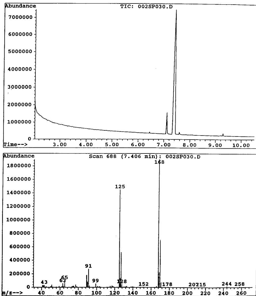
Figure 2. Mass spectrum of 3-chlorobenzorex
