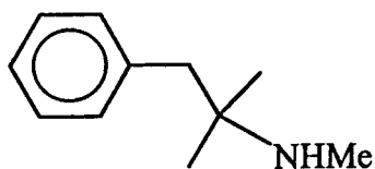
Mephentermine
