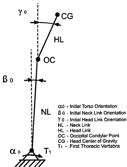
Figure 2. Two-pivot linkage mechanism representing head/neck structure.
