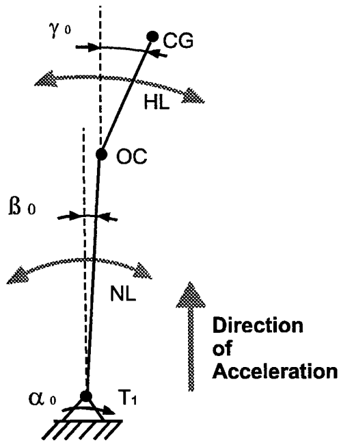
Figure 5. Schematic diagram showing direction of head/neck rotation for Mode E.
