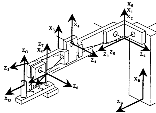
Figure 6. Freflex Kinematic Diagram
