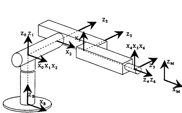
Figure 5. Merlin Kinematic Diagram
