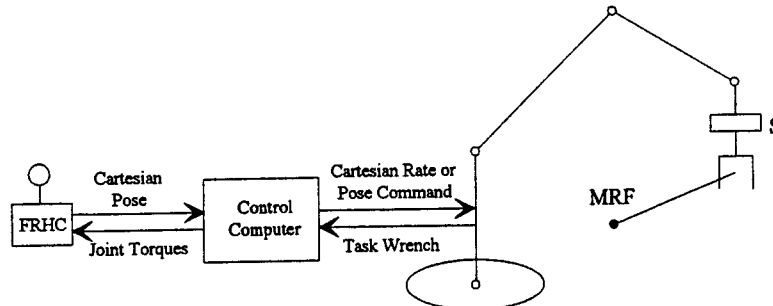
Figure 2. Force-Reflecting Teleoperated System
