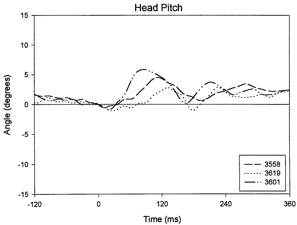
Figure 9. Sample experimental data for linear x-acceleration of the head and head pitch for Mode D.
