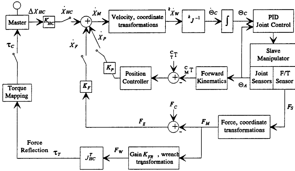
Figure 7. Telerobotic Control Architecture
