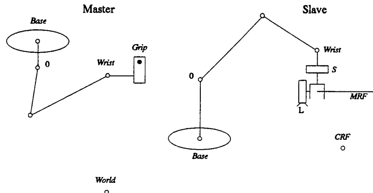
Figure 1. Master and Slave Coordinate Frames
