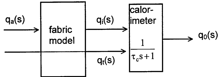
Figure 1: Block diagram of fabric and calorimeter models with inputs and outputs in Laplace ( s ) domain. q_a and q_t have been defined, q_i is the heat flux from the back side of the fabric and q_o is the calorimeter output.
