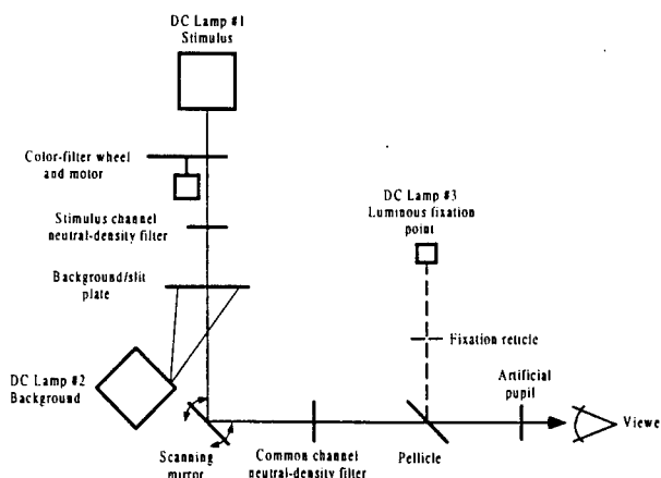
Figure 1. Simplified illustration of the FSC apparatus.
