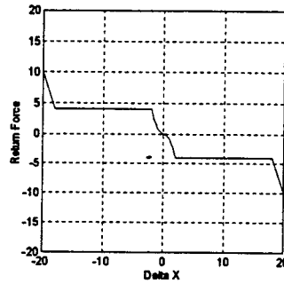
Figure 9. CFRTC for One Cartesian Axis
