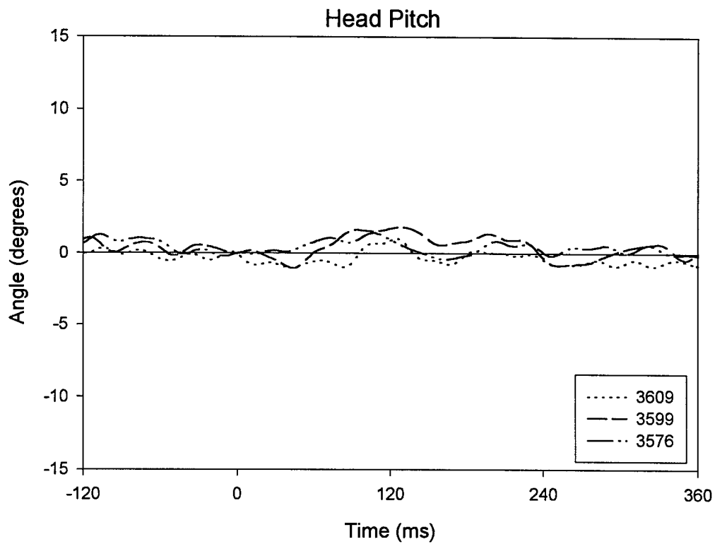
Figure 10. Sample experimental data for linear x-acceleration of the head and head pitch for Mode E.
