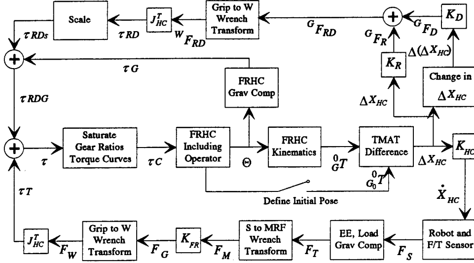
Figure 8. Cartesian FRHC Control Diagram
