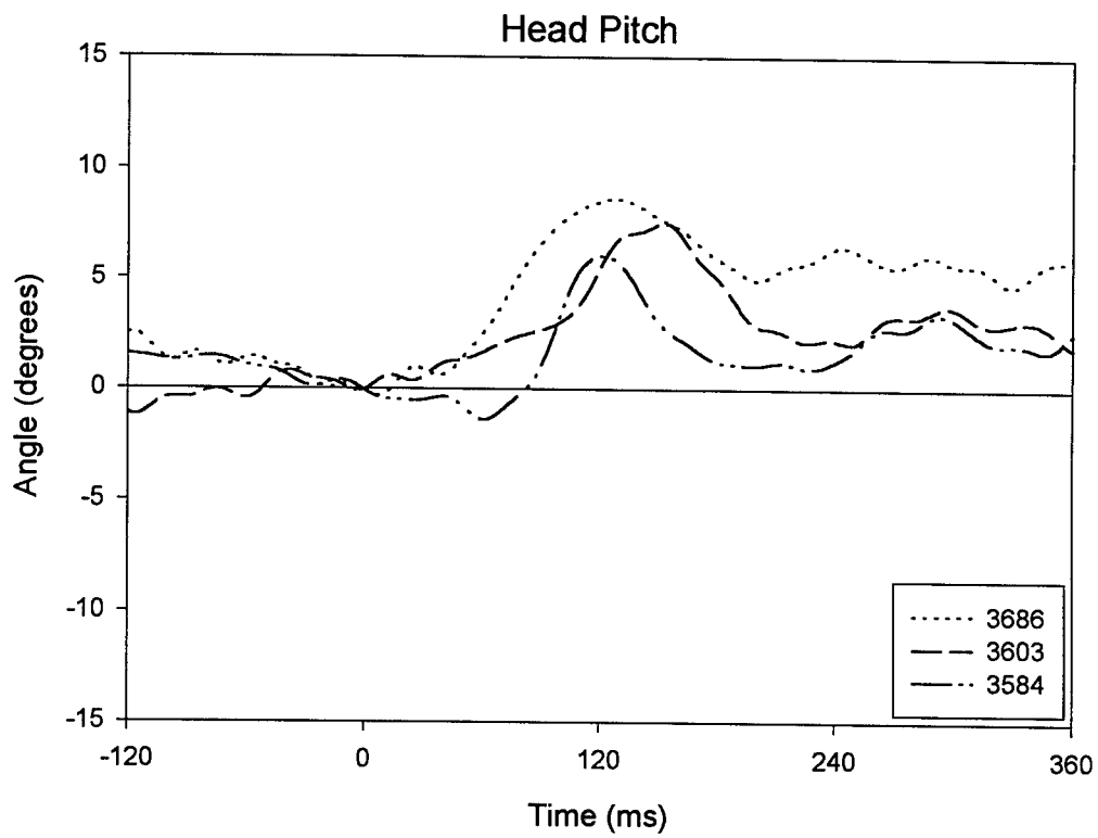
Figure 8. Sample experimental data for linear x-acceleration of the head and head pitch for Mode C.
