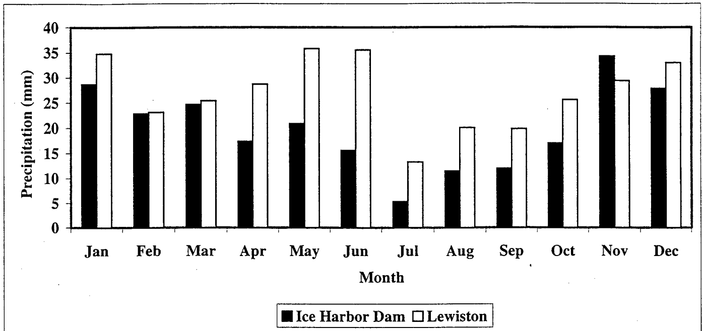
Figure 2-2. Average Monthly Precipitation Totals
