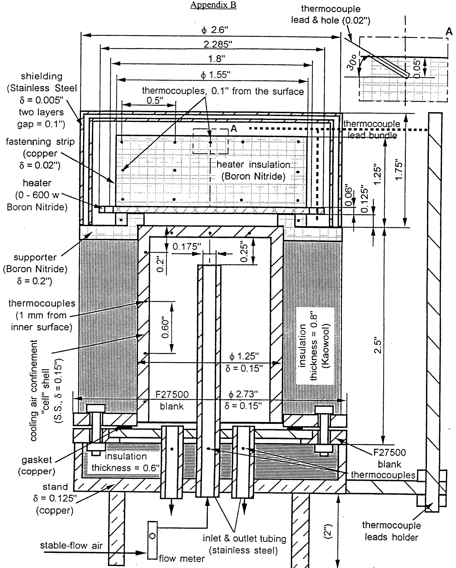
Calibration System for Cell Heating Device (4th Modification)
