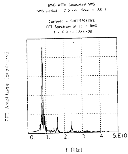
[b] FFT plot of BWO with Grid Heating Suppression
