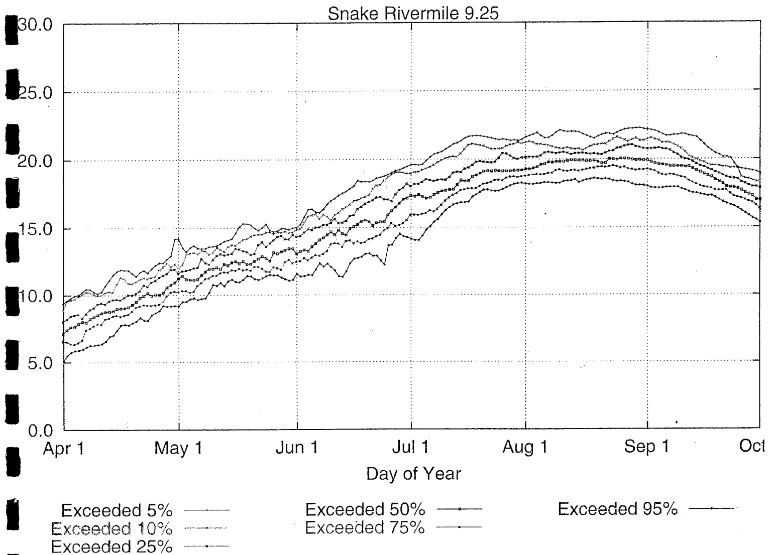
Figure 4-7. Summary of Mass 2 Simulated Temperature Variation at Snake River Mile 9.25 (near Ice Harbor Dam) during the Current Conditions Scenario
