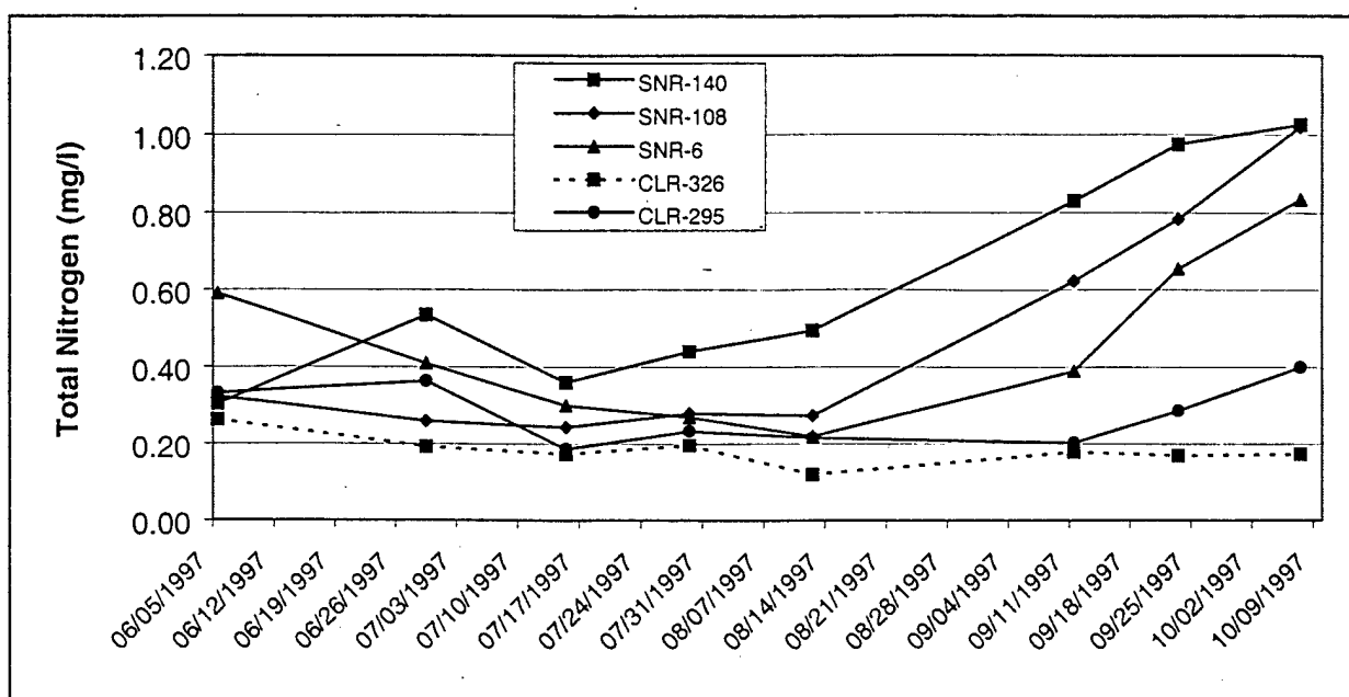
Figure 3-28. Total Nitrogen for Selected Sampling Stations in 1997
