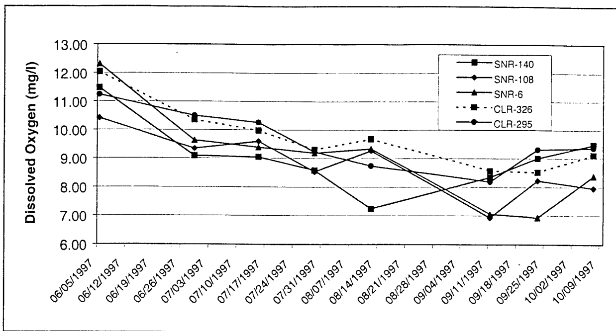
Figure 3-21. Dissolved Oxygen for Select Stations
