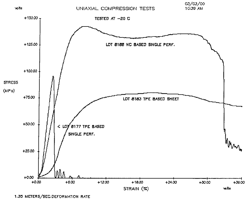
Figure 6. Stress vs. Strain Plot for Lots Tested at -20\text{ }^{\circ}\text{C} .
