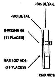
Figure 111 RPS Reference Standard for Joint Type III and IV
