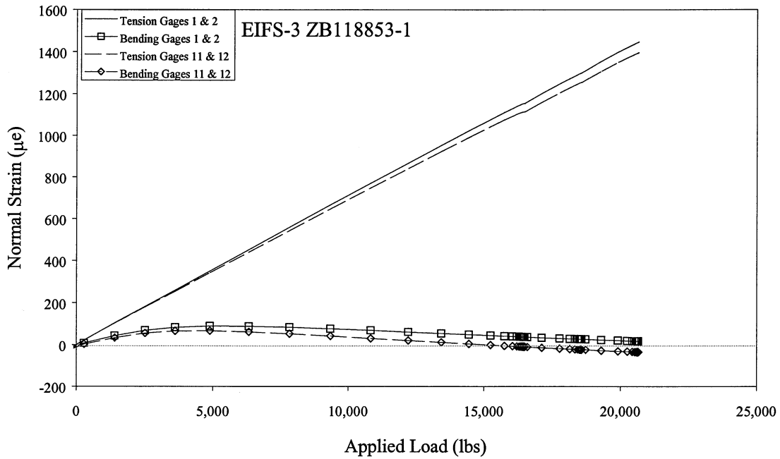
Figure 29 EIFS-3 Top Sheet Normal Strains
