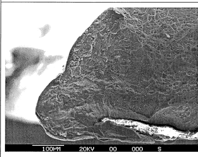
Figure 122 3C12R Nucleation Site
