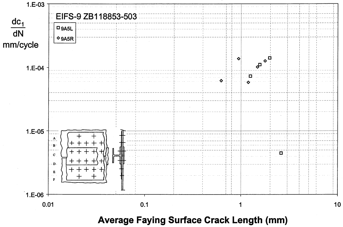
Figure 102 EIFS-9 Crack Growth Rates
