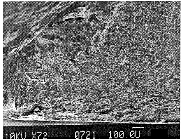
Figure 195 7A12R Nucleation Site, Macro View
