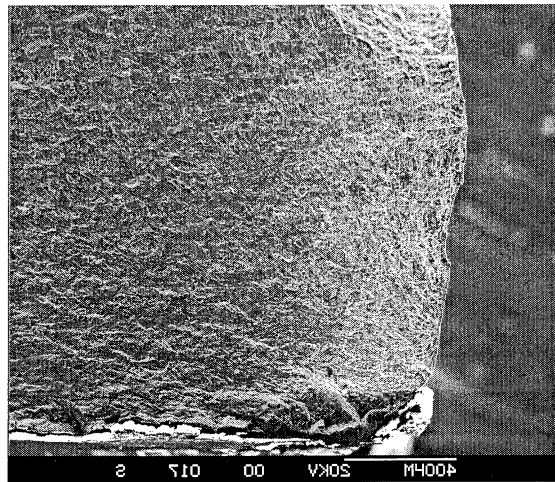
Figure 280 15E20L Nucleation Site
