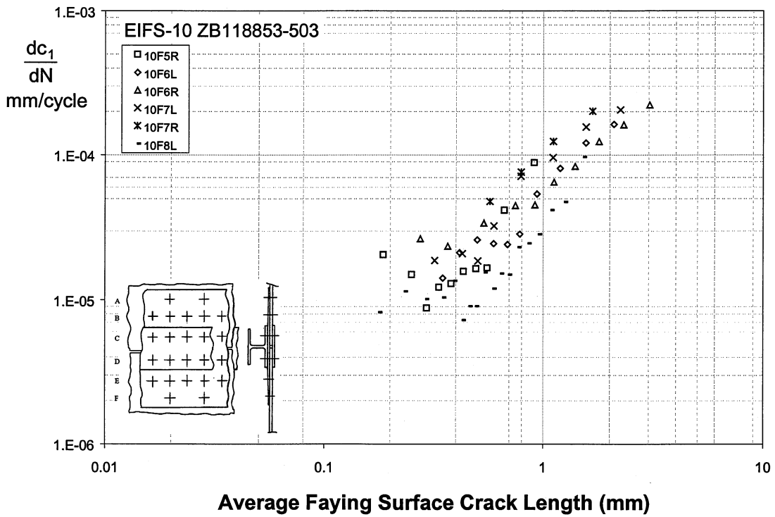
Figure 103 EIFS-10 Crack Growth Rates
