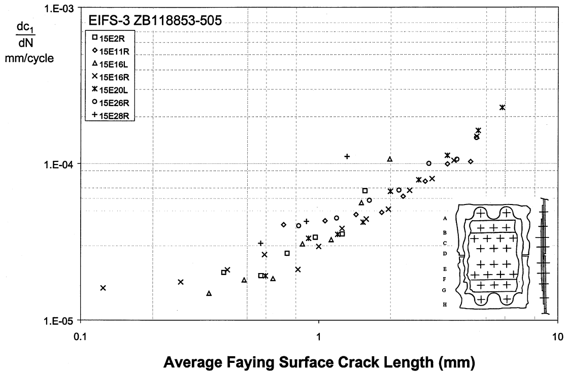
Figure 105 EIFS-15 Crack Growth Rates
