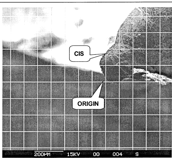
Figure 123 3C12R Nucleation Site
