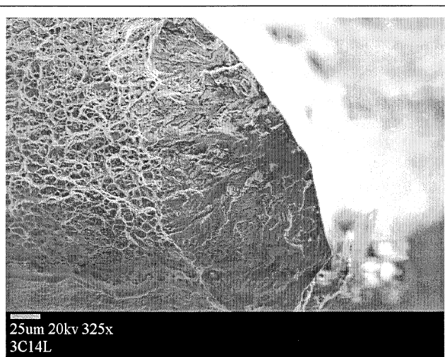
Figure 125 3C14L Nucleation Site
