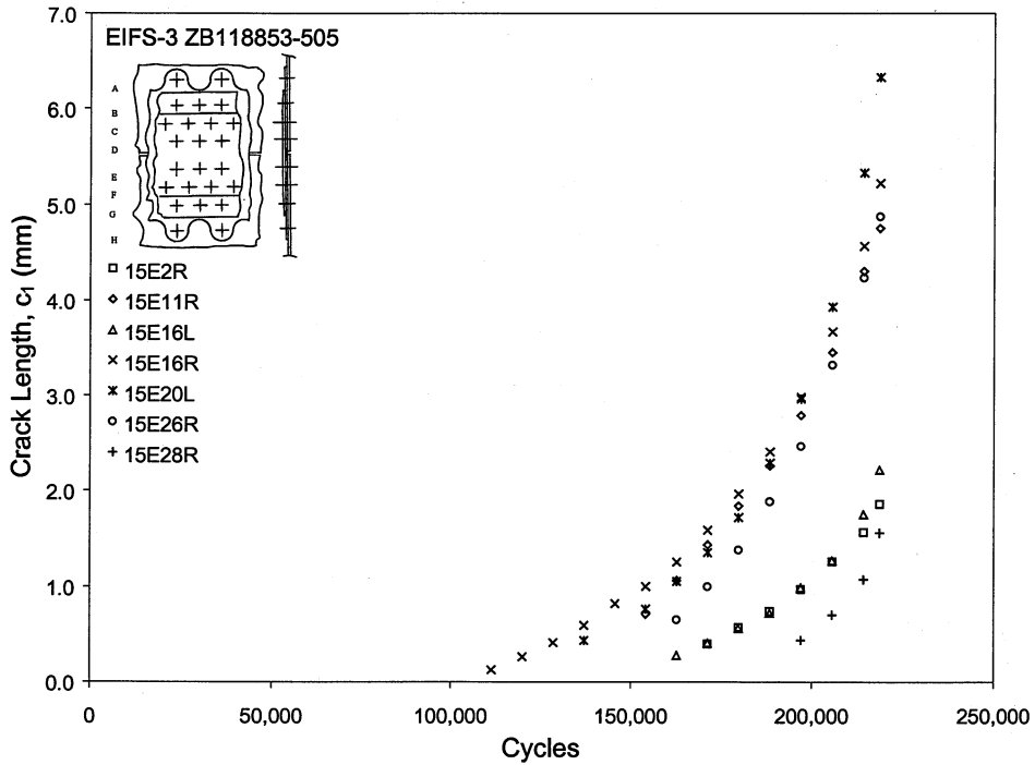
Figure 95 EIFS-15 Reconstructed Crack Histories
