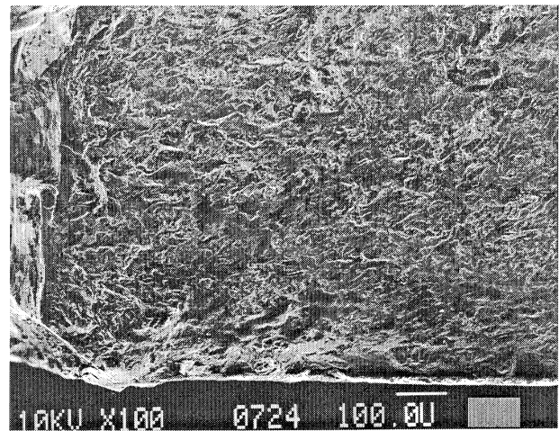
Figure 201 7A13R Nucleation Site, Macro View
