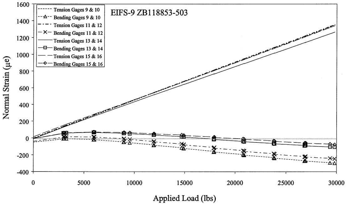
Figure 45 EIFS-9 Top Sheet, Critical Rivet Row Normal Strains
