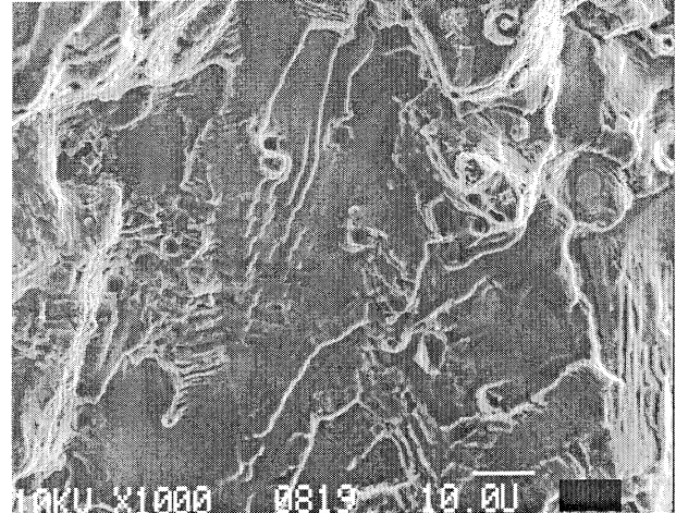
Figure 291 25 Minute 2% MicroClean™, Sonicate
