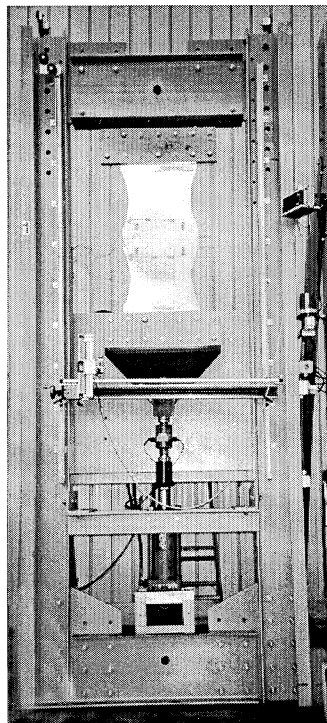
Figure 17 Joint Type III with Dogboned Skins
