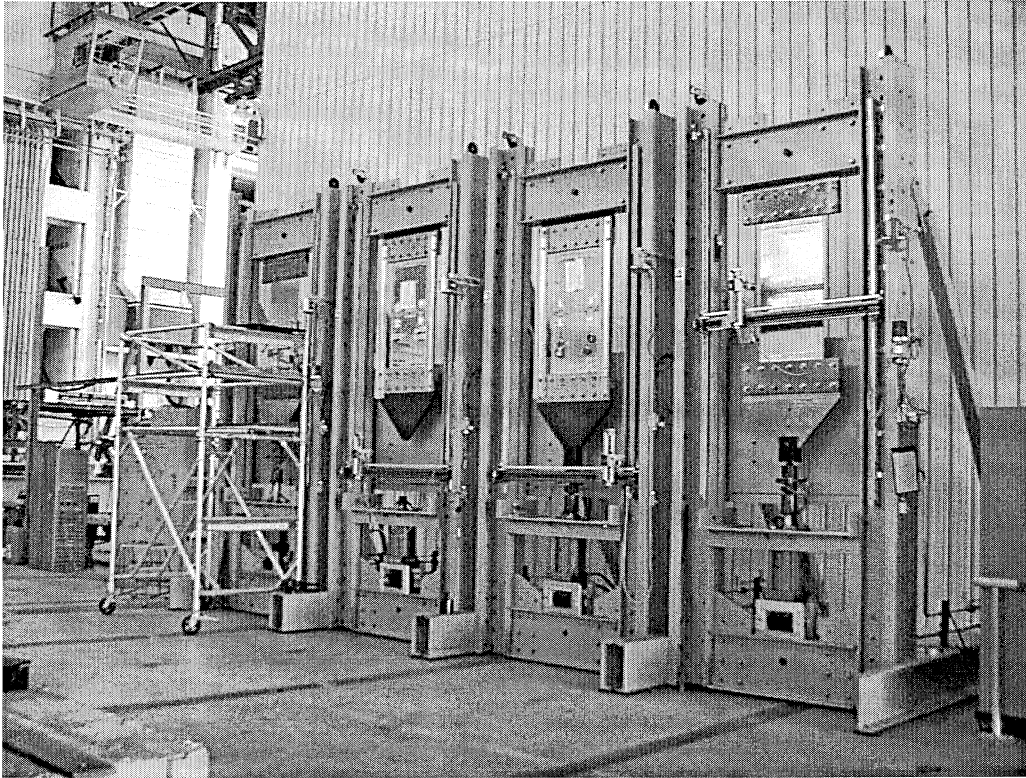
Figure 1 Air Force Research Laboratory Wide Panel Test Facility
