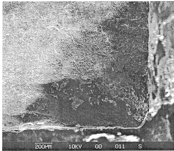
Figure 274 15E11R Nucleation Site
