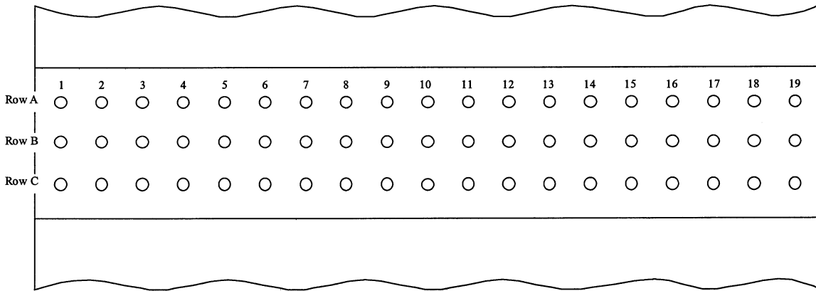
Figure 13 Strain Gage Locations for EIFS Type IV
