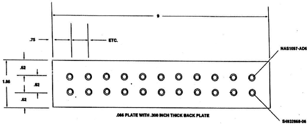
Figure 110 RPS Reference Standard for Joint Type I and II
