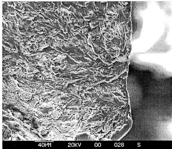
Figure 282 15E28R Nucleation Site
