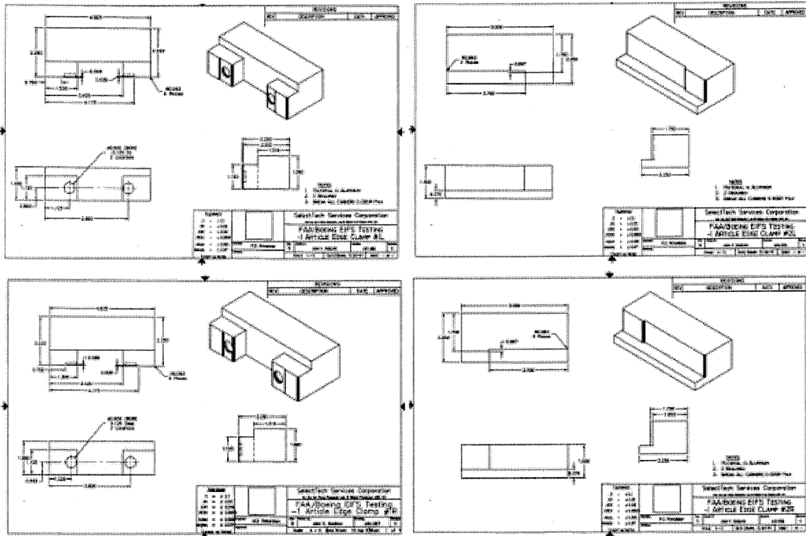
Figure 16 EIFS Type I and II Edge Blocks
