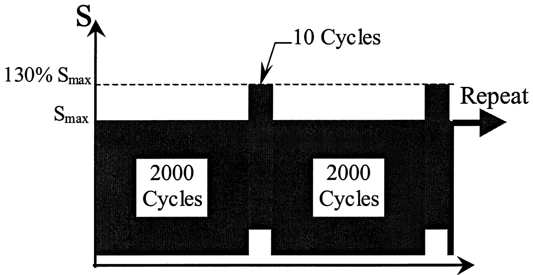
Figure 2 Overload Spectrum
