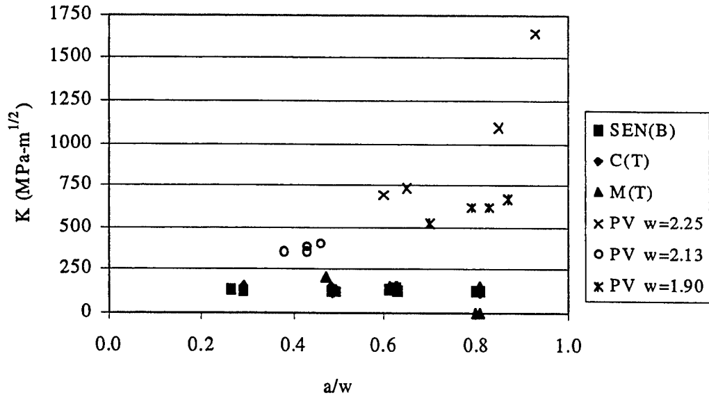
Figure 6. Calculated stress intensity for various configurations.
