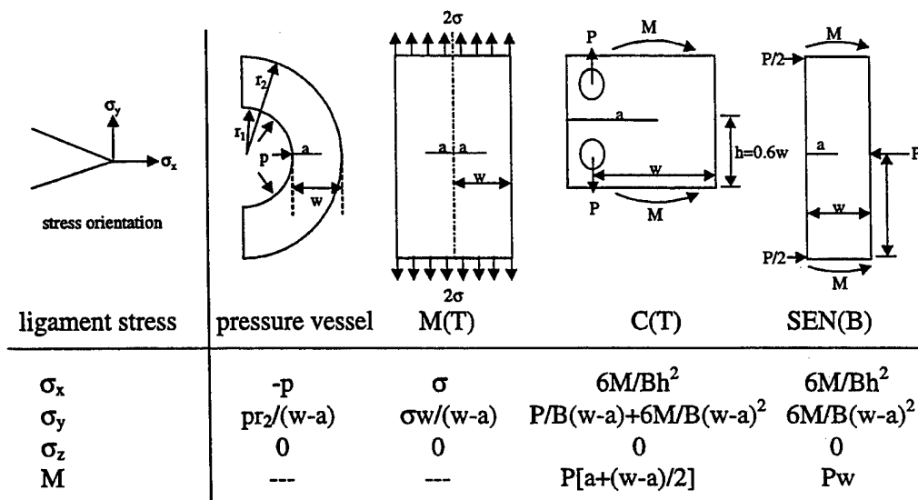
Figure 1. Ligament stresses for specimens investigated.
