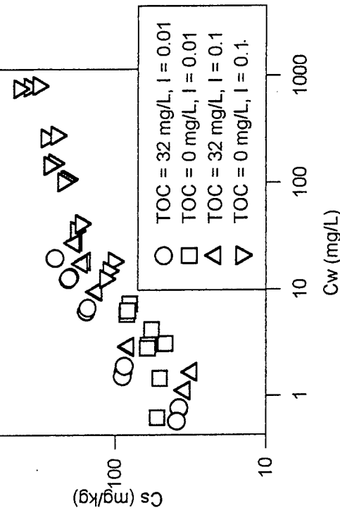
Figure 10. Sorption Isotherms: Blytheville
