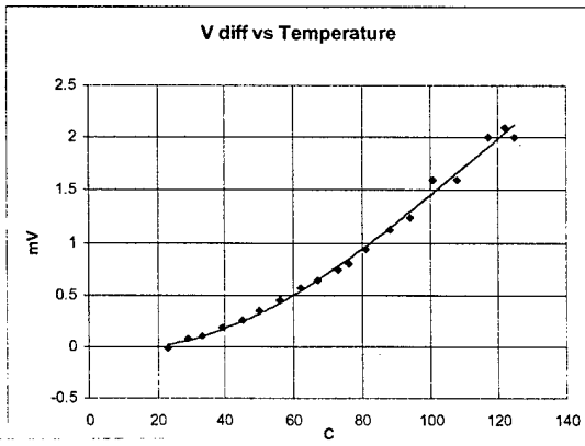
Figure 13a: Difference Response
