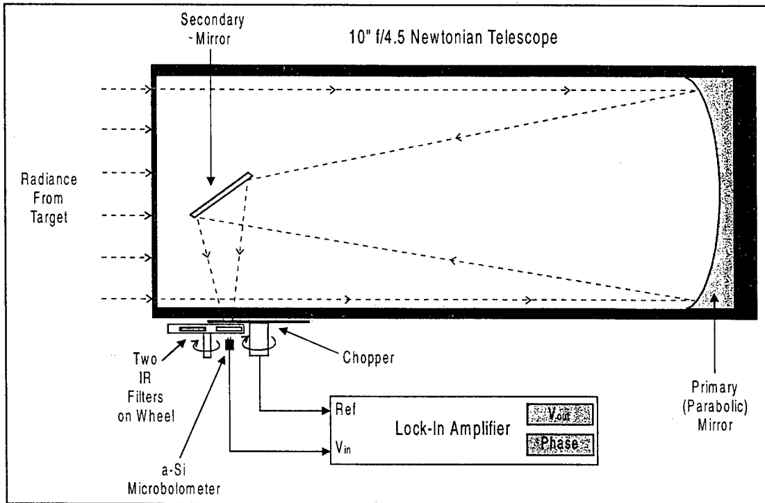
Figure 1: Phase I System Concept
