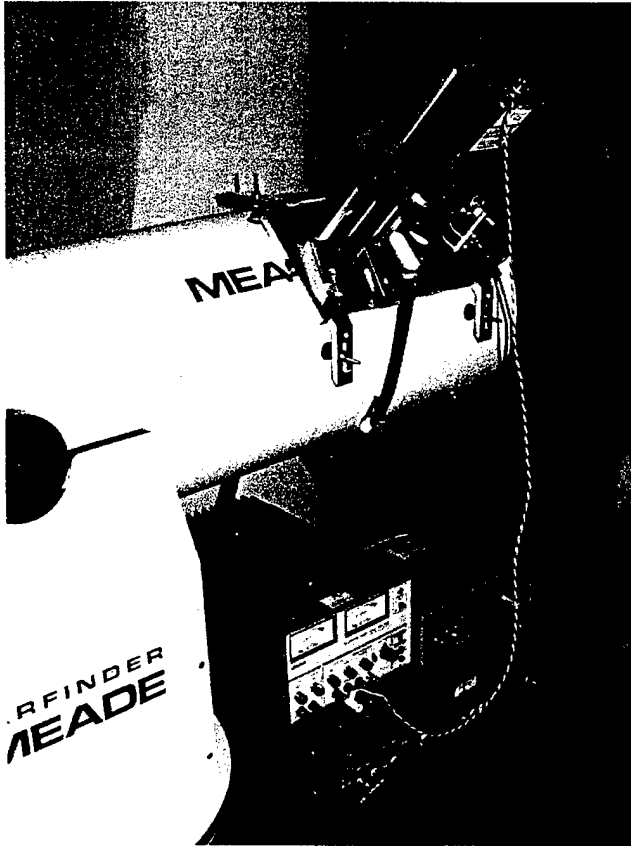
Figure 6: Phase I Telescope with Sensor Module
