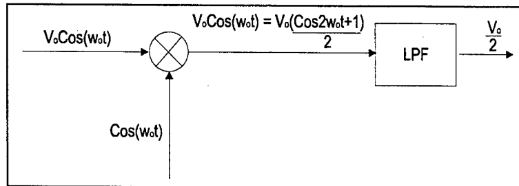
Figure 10: Synchronous Detection
