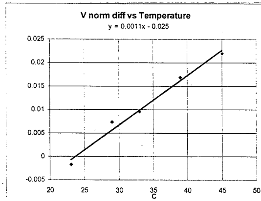
Figure 14a: Normalized Difference Response (low temperature)
