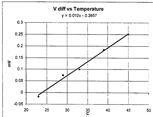
Figure 14a: Difference Response (low temperature)
