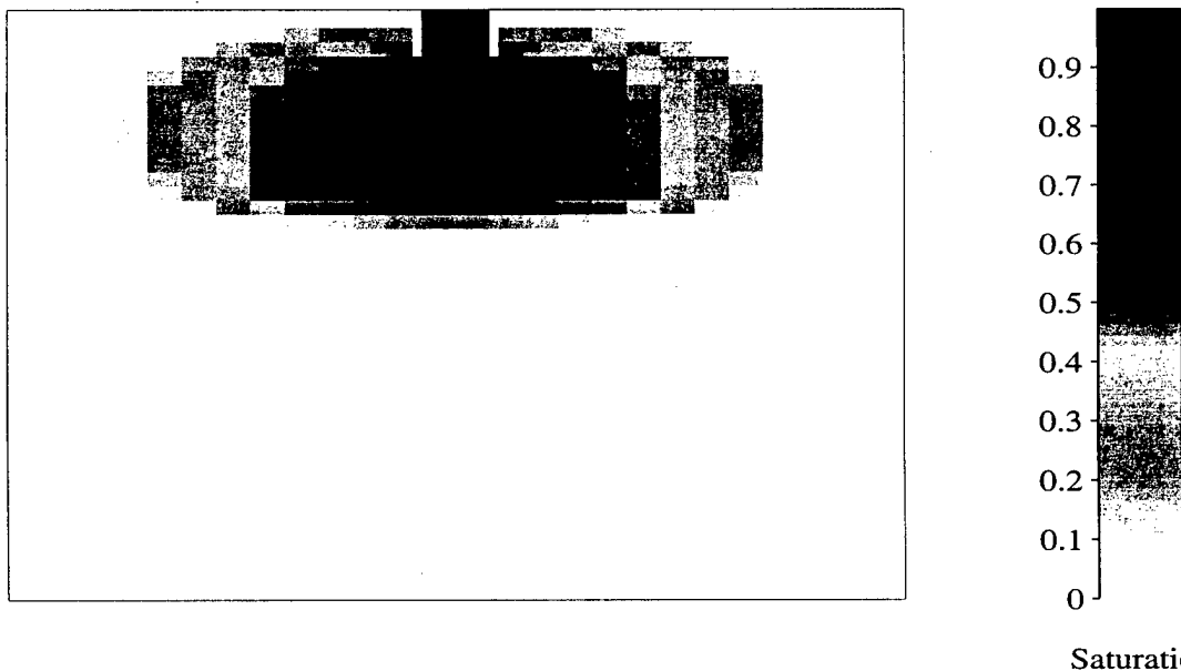
Figure 1. Simulation of PCE release at Borden site, after 8-hour constant flux injection.
