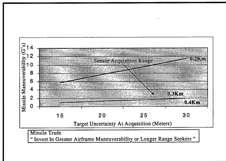
Figure 10 Required Missile Maneuverability
