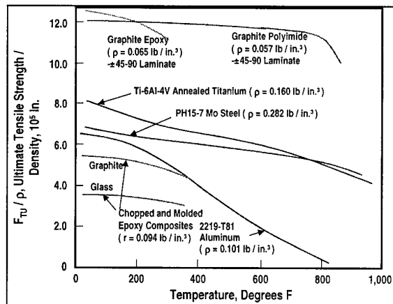
Figure 17. Composites Have High Structural Efficiency.
