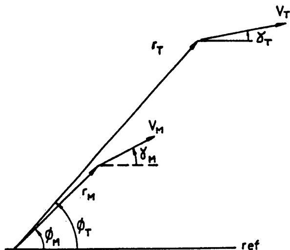
Figure 6. The kinematics of line-of-sight guidance.
