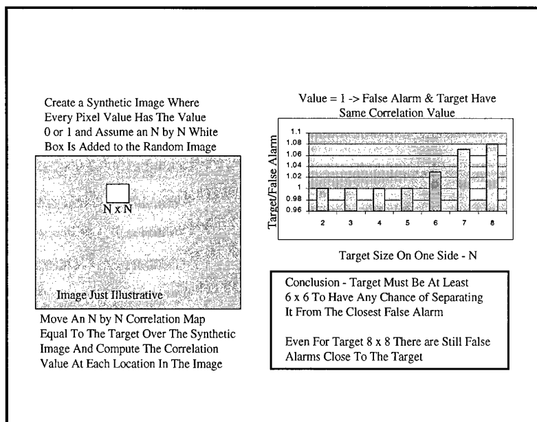
Figure 9 Number of Pixels on Target
