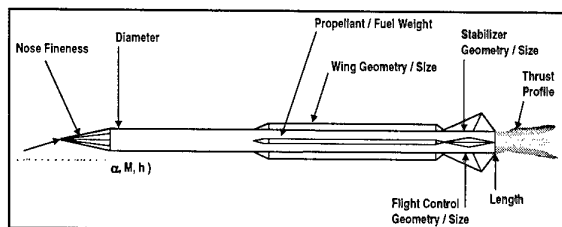
Figure 7. Aerodynamic Configuration Sizing Parameters.
