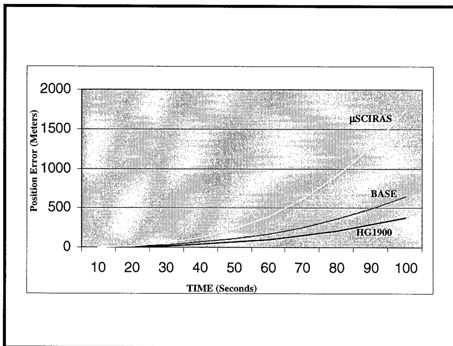
Figure 5. Representative Tactical Grade INS Position Growths
