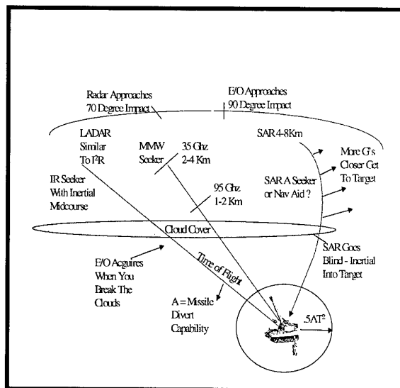
Figure 9 Airframe Seeker Trades
