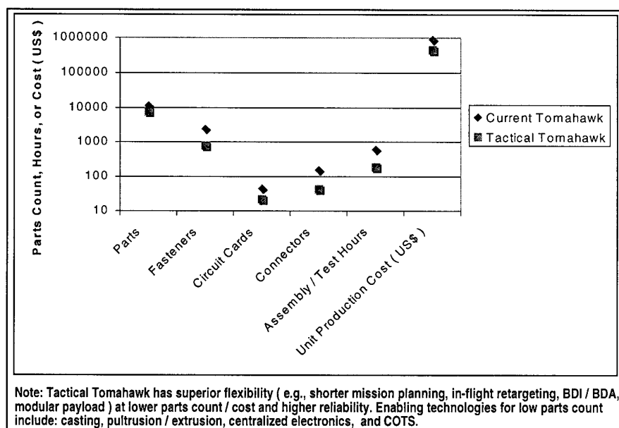
Figure 20. Low Parts Count Reduces Missile Cost.
