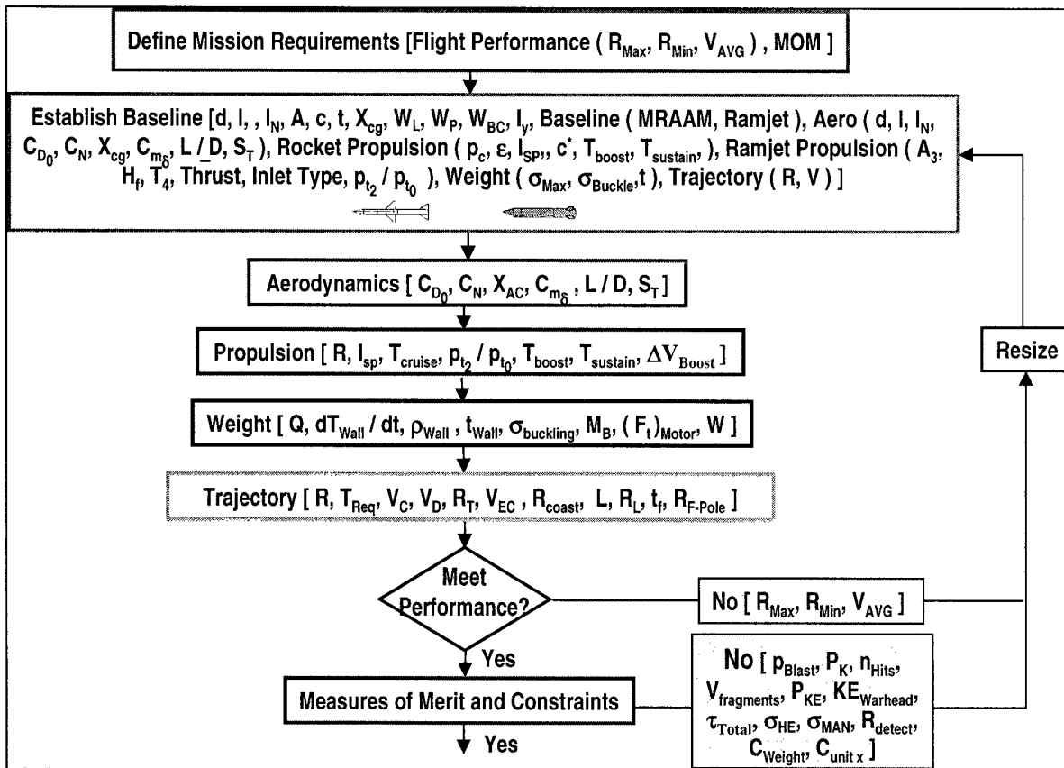
Figure 12. Tactical Missile Design (TMD) Spreadsheet Parameters.
