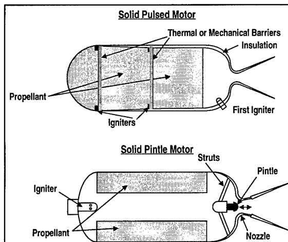
Figure 14. Thrust Magnitude Control Provides Efficient Thrust Management.
