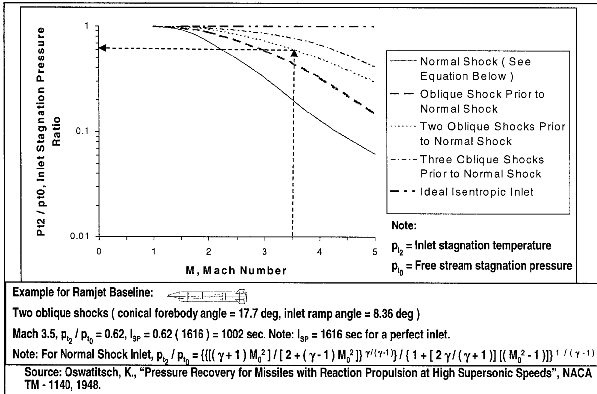
Figure 12. Ramjet Inlet/Airframe Integration Has Payoff.
