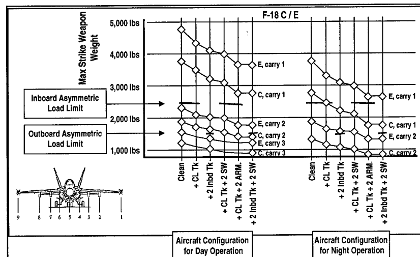
Figure 8. Light Missiles Enhance Firepower
