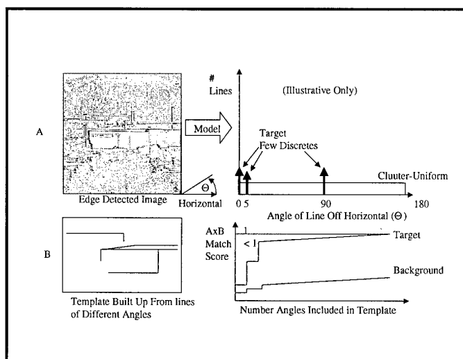
Figure 10 Template Complexity
