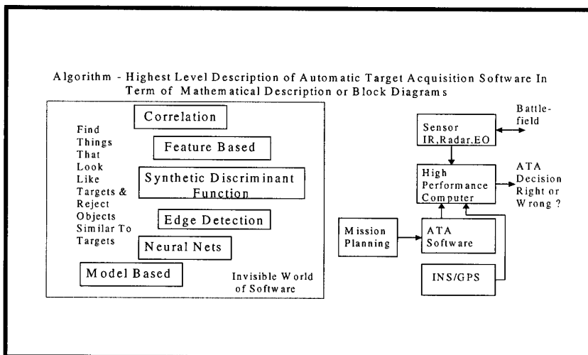
Figure 3 ATR Algorithms
