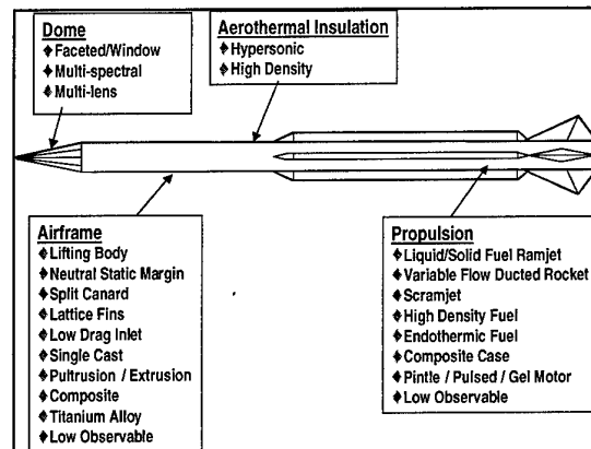
Figure 1. New Aeromechanics Technologies for Precision Strike Missiles.
