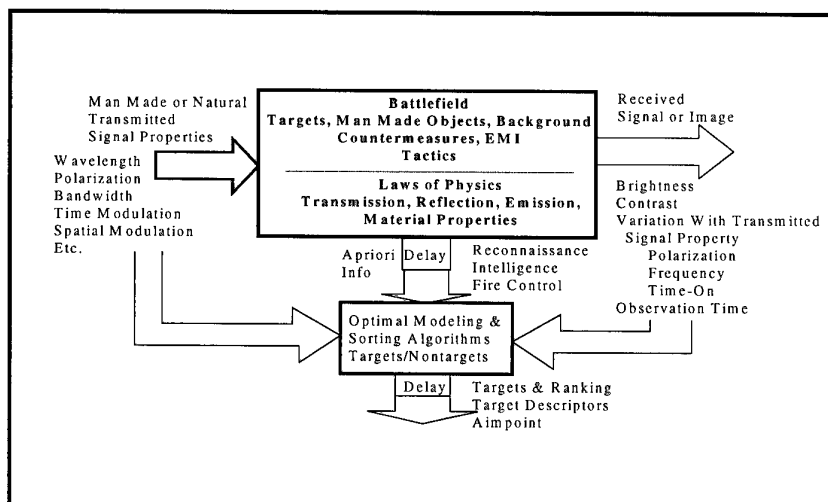
Figure 1 ATR High Level Architecture
