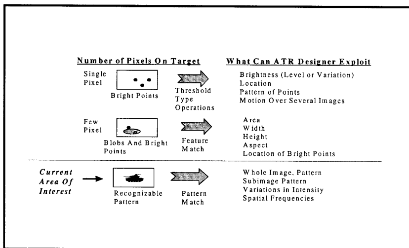
Figure 2 Levels of ATR
