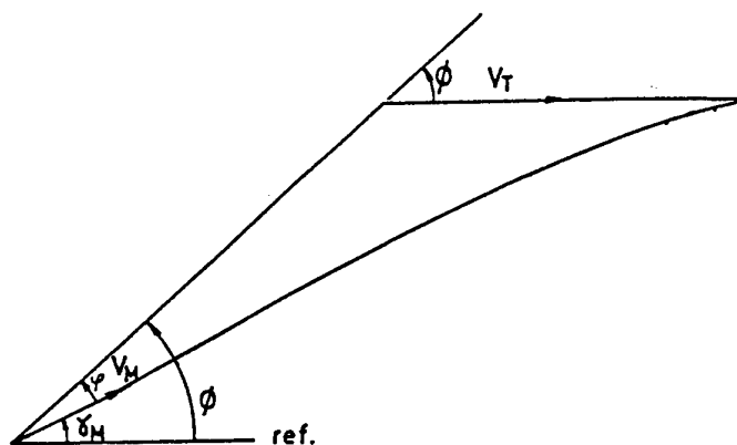
Figure 4. Proportional navigation, kinematics and definition of angles.
