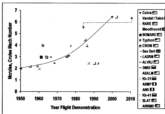
Figure 9. State-of-the-Art Evolution in Supersonic/Hypersonic Air Breathing Missiles.
