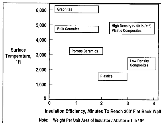
Figure 18. Composites Provide Light Weight Insulation.
