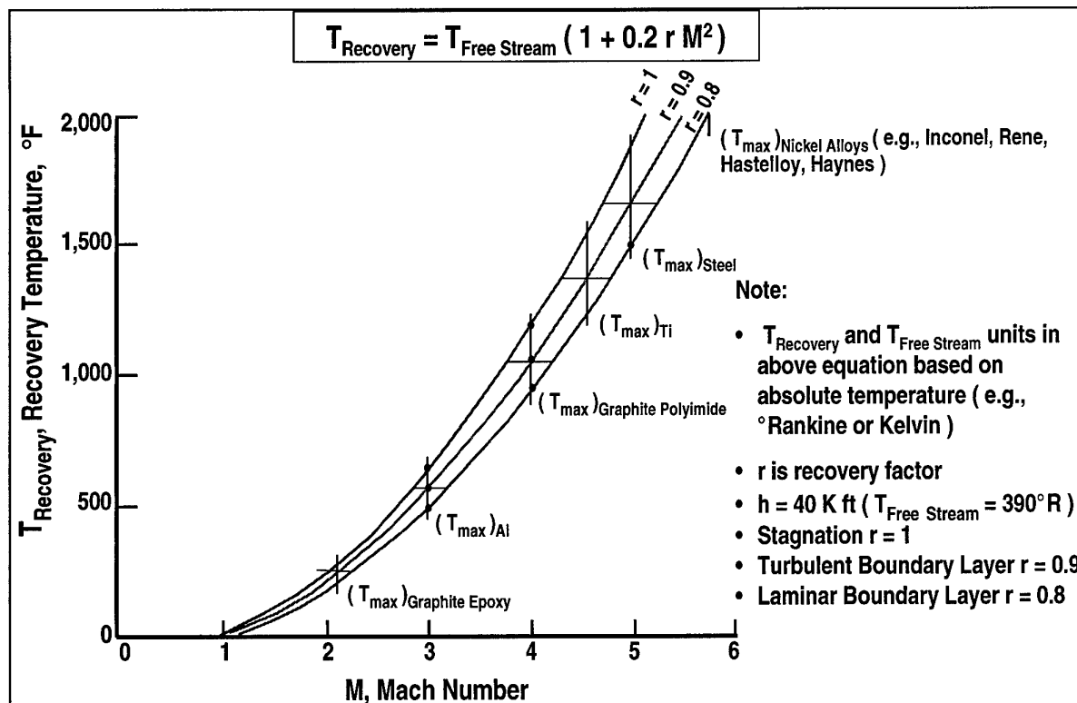
Figure 15. Hypersonic Missiles Require High Temperature Structure.
