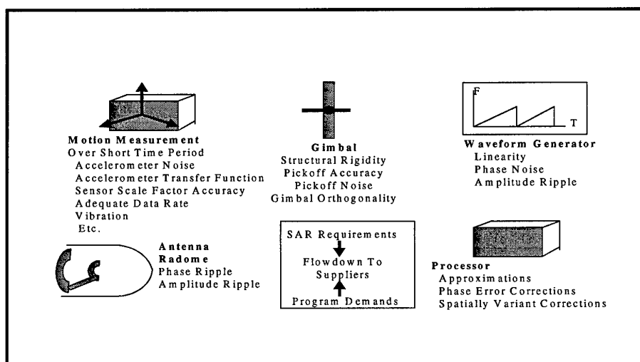
Figure 12 SAR Subsystems
