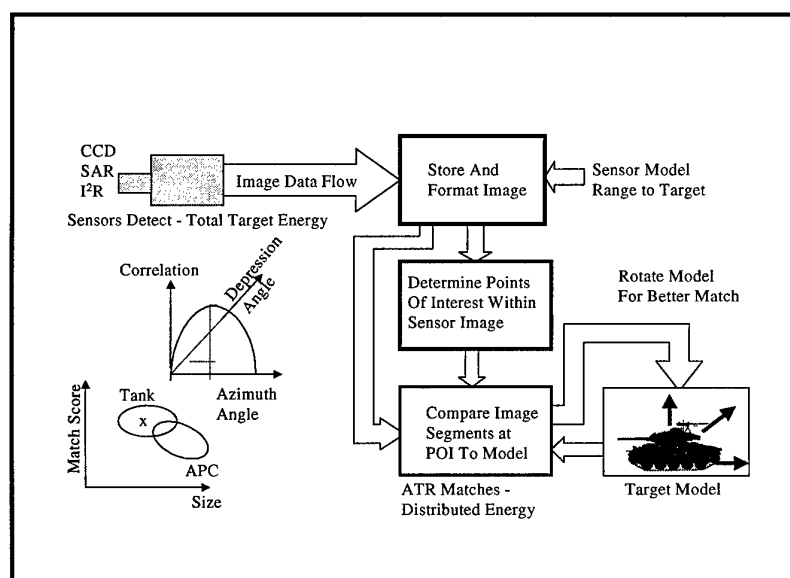
Figure 12 Detection in an ATR System
