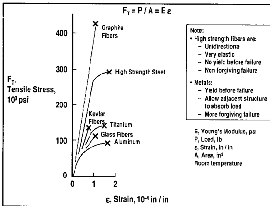
Figure 16. Composites Have High Strength.
