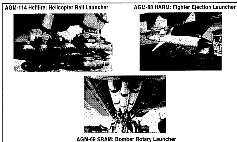
Figure 9. Precision Strike Missile/Aircraft Launch Integration Considerations.
