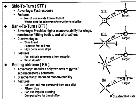
Figure 6. Bank-to-Turn Provides Higher Maneuverability
