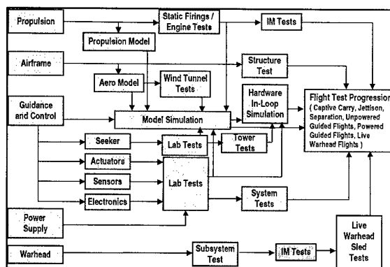
Figure 7. Design Validation/Technology Integration Is An Integrated Process.
