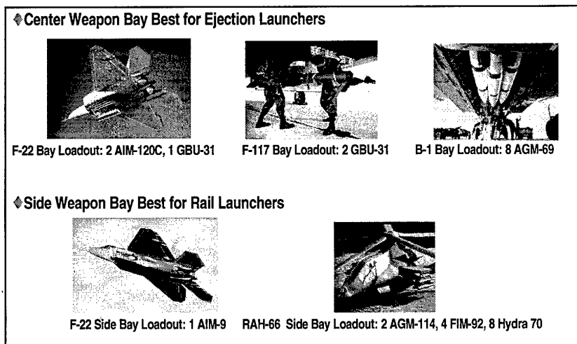
Figure 11. Internal Bay Carriage Has Low Observables.
