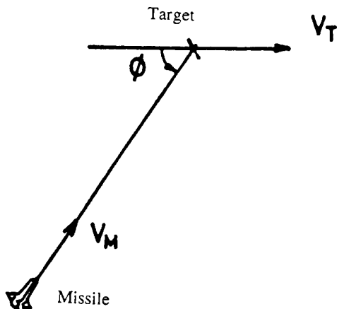
Figure 1. Velocity pursuit kinematics.
