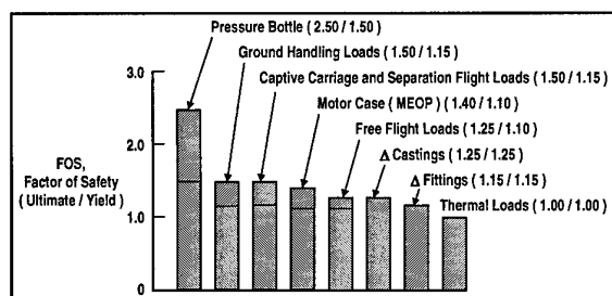
Figure 4. Missile Structural Design Is Driven by Safety.
