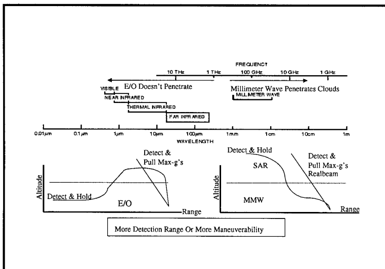
Figure 6 Cloud Penetration Problem
