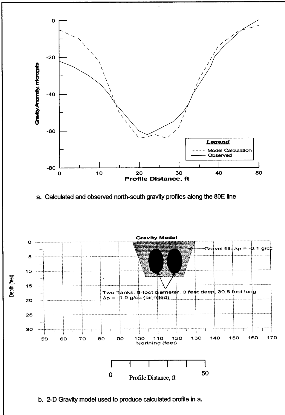
Figure 10. Observed and calculated gravity profiles and 2-D model of UST's and trench
