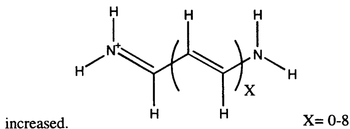
Figure 1. Simple Cyanines
