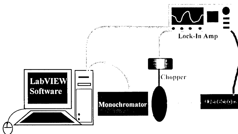
Figure 5: Testing Set-Up
