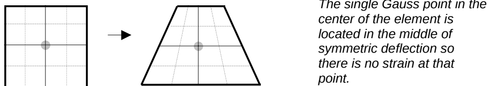
Figure 31. Gauss Point Location in Reduced Order Bending Mode.
