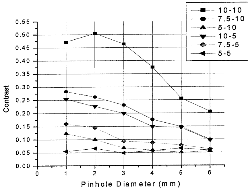
Figure 3. Simulated Results. Contrast versus pinhole diameter. Contrast improves with smaller pinhole diameter due to increased spatial resolution and thus less partial volume effect.
