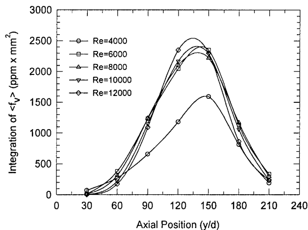
Fig. 6. Axial profiles of integrated soot volume fraction \sum \langle f_v \rangle as obtained from \sum \langle f_v \rangle = \pi \left( \int_0^r \langle f_v \rangle r dr + \int_{-r}^0 \langle f_v \rangle r dr \right) for both positive (+r/d) and negative (-r/d) directions from the flame centerline.
