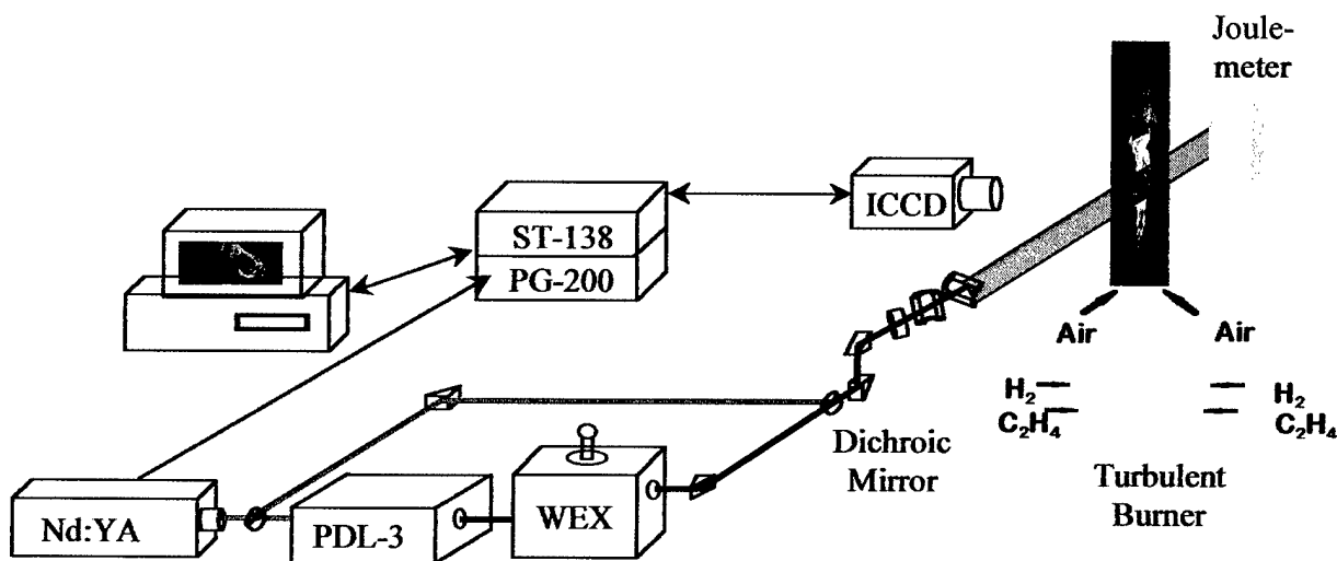
Fig. 2. Experimental set-up for 1-D or 2-D imaging of turbulent jet/air diffusion flames. OH \cdot is excited by the laser wavelength of 283.55 nm corresponding to Q 1 (8) of the OH \cdot band. Qualitative measurements of PAH are also obtained by de-tuning the laser off the OH \cdot transition and observing the fluorescence signals. The interference filter and camera gate width for LII measurements are 400 \pm 12.5 nm, 50 ~ 80 ns initiated directly after the laser pulse, respectively. The OH \cdot and PAH signals are collected from 300 nm to 380 nm with a 15 ns detection gate width. Simultaneous measurements of planar laser-induced incandescence (LII) of soot and laser-induced fluorescence (LIF) of OH \cdot and PAH can also be carried out using one ICCD camera system.
