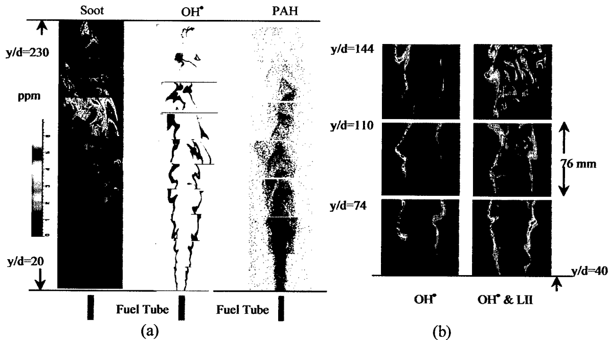
Fig. 3. General structure of soot, \text{OH}\cdot and PAH fields (a) and joint measurements of soot and \text{OH}\cdot (b) at Re=12000 (2.18 mm I.D. fuel tube burner). For (a), each image section is collected at a different time and pieced together to give a composite representation of the flame. For the joint measurements of soot and \text{OH}\cdot in (b), a \text{OH}\cdot band filter was used for both signals with a wide gate width of \sim 80 ns. The large signal ratio between LIF to LII measurements was used to discriminate between the two signals since both signals are captured on the same ICCD.
