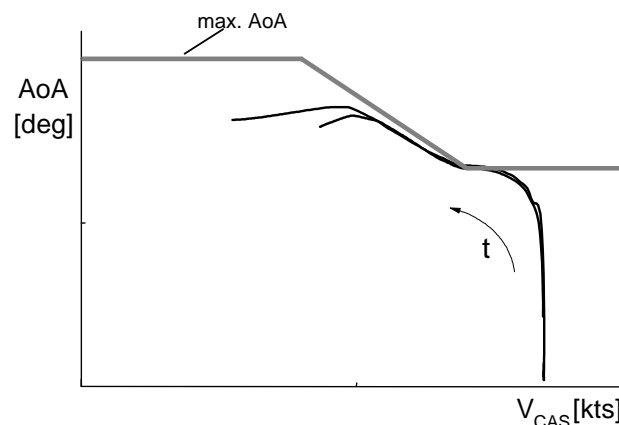
Figure 5.1.3: Simulation of deceleration flights with digital flight controller (full back stick)
