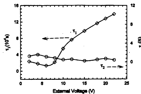
Fig. 10. The fitted lifetime \tau_1 (◊) of excited protons and the rate constant \tau_2 (●) according to Eq. 11 as functions of the external voltage. The flash power and flash period are 129.0 mW and 10 s, respectively.
