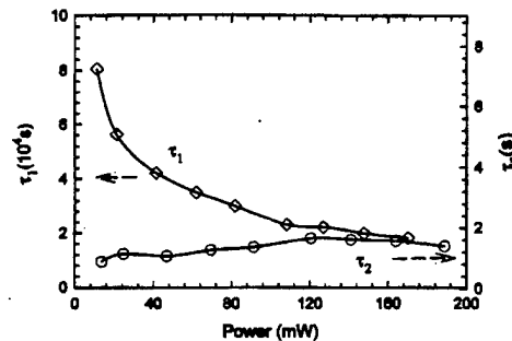
Fig. 9. The fitted lifetime \tau_1 (◊) of excited protons and the rate constant \tau_2 (●) according to Eq. 11 as a function of the flash power. The external voltage and flash period are 20 V and 5 s, respectively.
