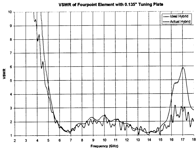
Figure 1.2.3-1 Measured VSWR at hybrid of a Fourpoint antenna.
