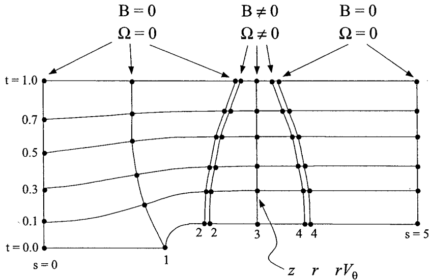
Figure 3-3: Field parameter s, t grid for an open propeller on a straight shaft, showing doubled t profiles at blade leading and trailing edge.
