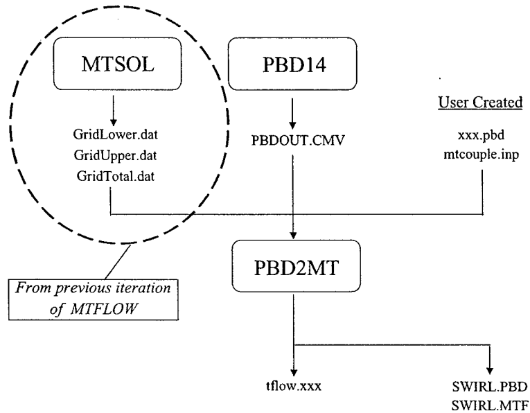
Figure 3-1: Program order and file passing when running PBD to MTFLOW. The end product is the ascii file tflow.xxx , which is the required input for MTFLOW.
