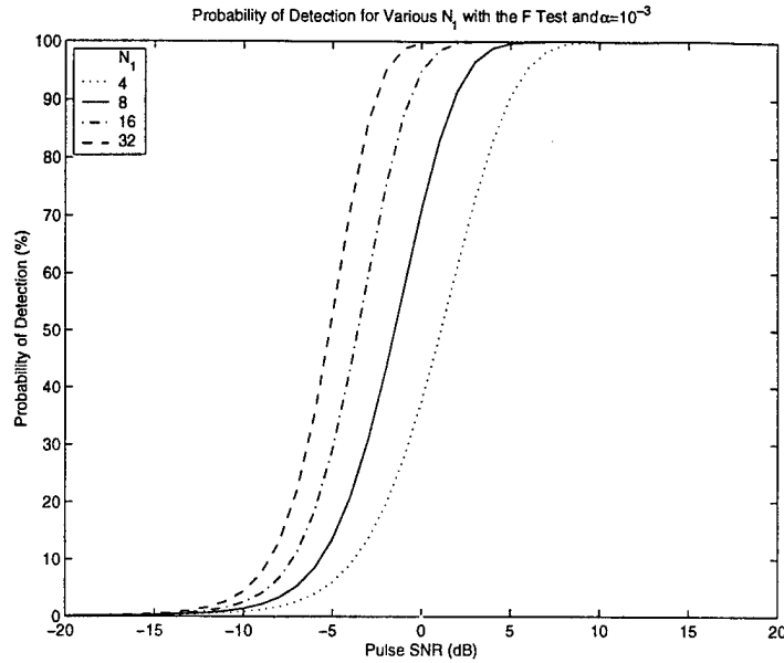
Figure 3.4 Probability of detection (power) for various length of the Z_{N_1} observation interval with N_0 = 64 .
