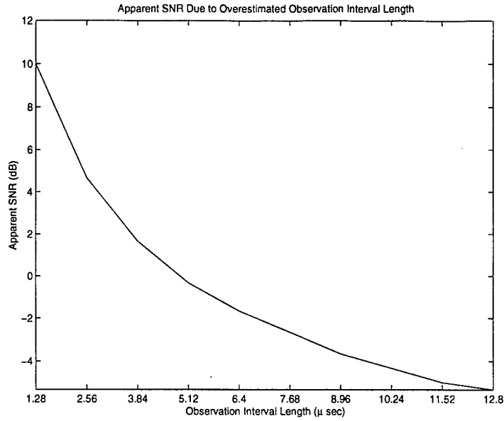
Figure 3.5 Apparent SNR of a 10-dB pulse 1.28 \mu s long caused by overestimating the observation interval length up to 10 times.
