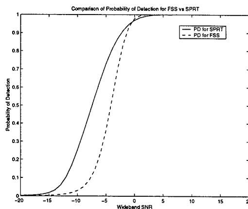
(b) -10-dB Design SNR and 20 Sample Design ASN
