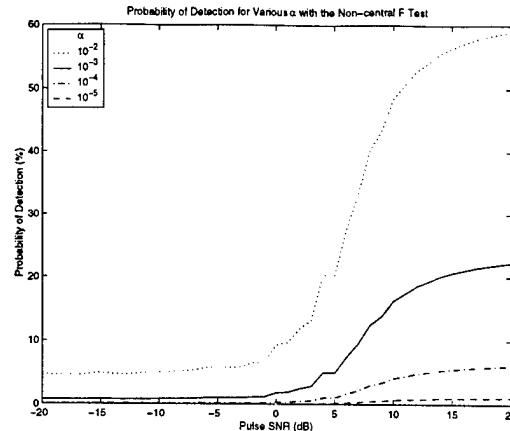
(b) Power
