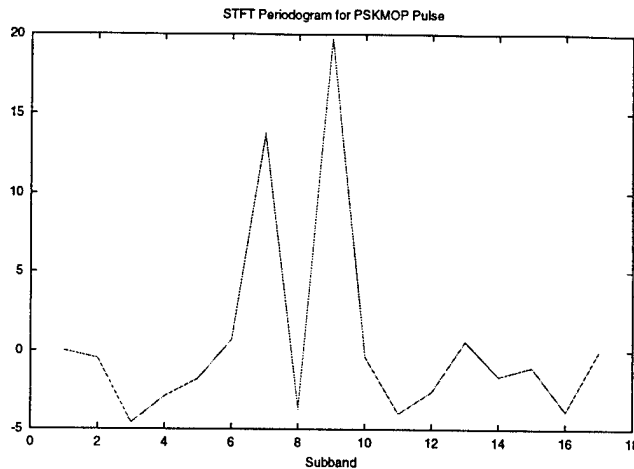
Figure 5.2 STFT from a PSKMOP pulse.
