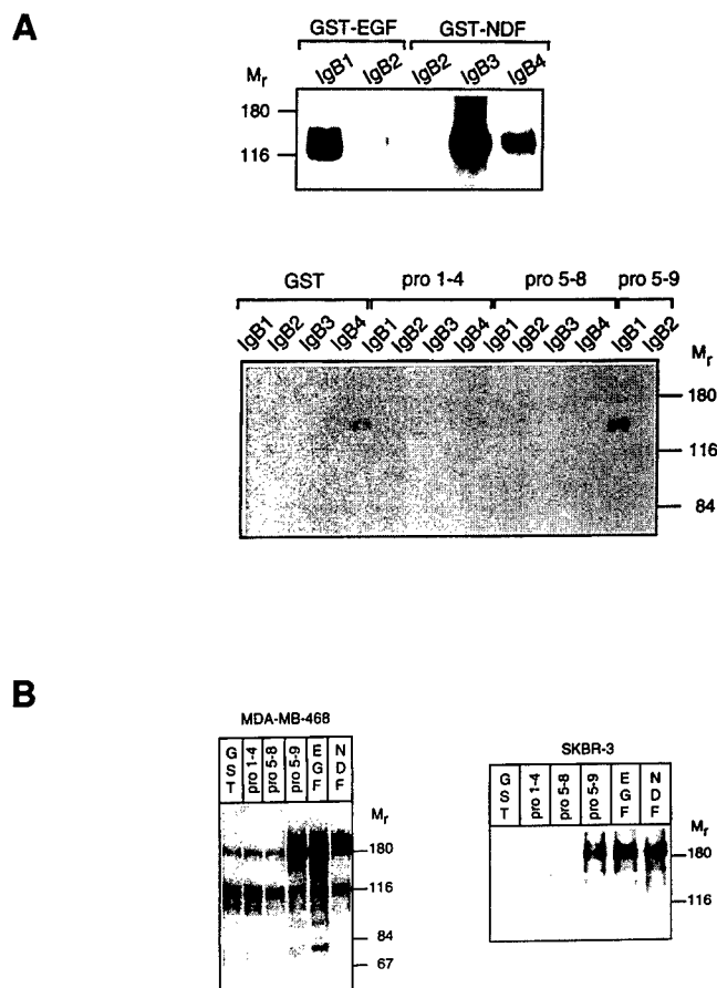
FIG. 4. Activation of ErbB receptors by EGF-like motifs of human proEGF. ( A ) GST fusion proteins containing EGF-like motifs 1–4, 5–8, or 5–9 of the EGF precursor were immobilized on glutathione-agarose beads. For control, GST fusion proteins containing EGF or NDF were used. The beads were incubated for 1 h at 4°C with conditioned media containing 1 \mu g of the indicated IgB protein. Protein complexes were immunoblotted with an anti-human Fc antiserum for detection of bound IgBs. ( B ) Monolayers of the indicated human breast cancer cell lines were incubated, for 10 min at 37°C, in the presence of 100 ng/ml GST fusion proteins or 5 ng/ml ligands (EGF or NDF). Receptor activation was detected by an antiphosphotyrosine antibody.
