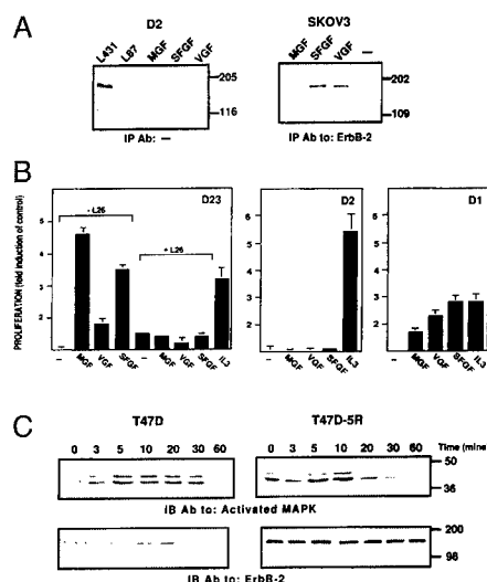
FIG. 5. Viral peptides recruit ErbB-2. ( A ) Phosphorylation of ErbB-2 by viral peptides [vaccinia virus growth factor (VGF), Myxoma virus growth factor (MGF), and SFGF] and antibodies (L87, L431) was examined as described in the legend to Fig. 1. ( B ) IL-3-deprived D23 cells were stimulated by viral peptides in the presence (+L26) or absence (–L26) of a class II mAb to the human ErbB-2 (Left). Cells singly expressing ErbB-2 (D2) or ErbB-1 (D1) served as negative and positive controls for ligand activity, respectively. Proliferation induction was determined by the 3-(4, 5-dimethylthiazol-2-yl)-2,5-diphenyl tetrazolium bromide assay as described in the legend to Fig. 2. For control of endogenous proliferation signals, we incubated cells with IL-3. ( C ) The effect of ErbB-2 on downstream activation by SFGF was examined in cells that do (T47D) or do not (T47D-5R) express ErbB-2 on their surface. A time response of activation was detected in whole cell lysates by immunoblotting with an antibody against activated MAPK. The amount of ErbB-2 was verified by immunoblotting the upper part of the membrane with an antibody against the receptor.
