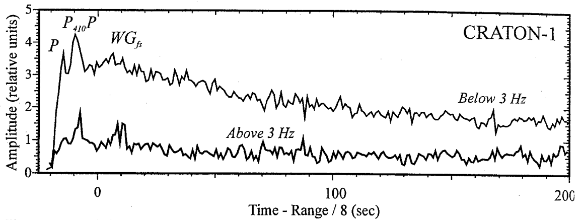
Figure 8. Records from PNE CRATON-1 in the West Siberian basin averaged and plotted in the same way as QUARTZ-4 records in Figure 3. Due to lower frequency content of these records, the frequency band separation is performed at 3 Hz instead of 5 Hz in Figure 3. Note that even without correcting for coda build-up, the WG_{fs} is weaker than P_{410}P and also much weaker than in the records from QUARTZ-4 (Figure 3). Also note the longer codas and increased high-frequency content of WG_{fs} (compared to WG ), in contrast to Figure 3. These differences suggest regional variations in WG propagation characteristics and lower crustal attenuation within the Siberian craton.
