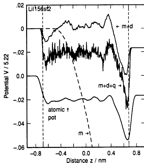
Fig. 8. Electric potential drop across a neutral solution consisting of one lithium ion \text{Li}^+ , one iodide ion \text{I}^- and 156 ST2 waters next to an immersed electrode. Potential due to atom method shifted by -0.04 . Potential from: ions only m , ions and water dipoles m + d , ions and water dipole and quadrupole m + d + q . Note that the potential m + d + q is almost the same as that calculated from atomic charges. There is no net image charge on the metal. Metal electrode on right-hand side, restraining wall on the left. Image plane at z = 0.931 nm. Wall potentials go through zero at |z| = 0.682 nm.
