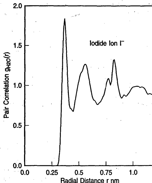
FIG. 6. The pair correlation function for water distributed around the adsorbed \text{I}^- ion. Only the distribution within the bulk cone (half-angle of 60^\circ ) is shown. There are no water molecules between the iodide and electrode in the surface cone.
