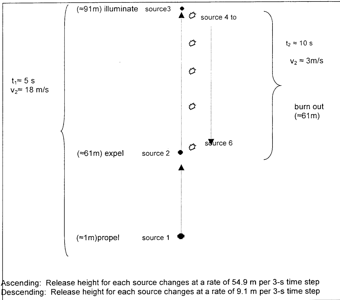
FIGURE 1: SCHEMATIC DIAGRAM OF THE TRAJECTORY OF THE M125A1
