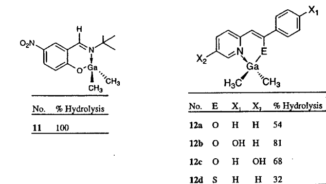
Figure 2. Structure of gallium complexes and percent hydrolysis (after 12–24 h with 1000-fold excess of water in acetone- d 6 monitored by 1 H NMR).
