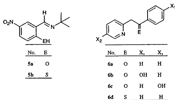
Figure 1. Ligand precursors.
